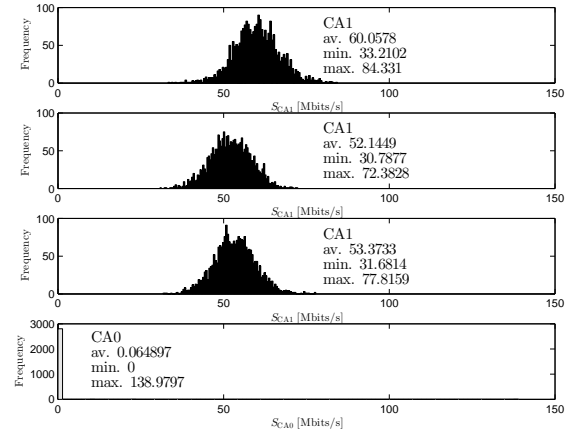
Fig. 7. Histograms of throughput (measured at 1s intervals with iperf ) for Scenario 2 ( n_{CA1} = 3, n_{CA0} = 1 ).
