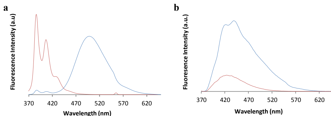
Fig. 4. Fluorescence emission spectra of L (6 \mu\text{M} in MeCN). a. PIC (blue, \lambda_{\text{ex}} 343 nm) and PIM (red, \lambda_{\text{ex}} 274 nm); b. AIC (blue, \lambda_{\text{ex}} 364 nm) and AIM (red, \lambda_{\text{ex}} 364 nm).
