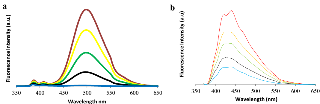
Fig. 8. Fluorescence emission spectra of L (red; 6 \mu\text{M} , MeCN), a. PIC ( \lambda_{\text{ex}} 343 nm) and b. AIC ( \lambda_{\text{ex}} 364 nm), following titration of 2 (yellow), 5 (green), 10 (black) and 20 (blue) equivalents of \text{Cu}(\text{ClO}_4)_2 to the host solutions.
