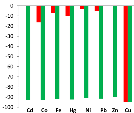
Fig. 7. Percentage change in the intensity of maximum fluorescence emission of PIC ( 6 \mu\text{M} , MeCN, \lambda_{\text{ex}} 343 nm; \lambda_{\text{max}} 498 nm); Red, upon the addition of 20 equiv of metal perchlorates; Green, upon the further addition of 20 equiv of copper perchlorate to the PIC -metal perchlorate solutions.
