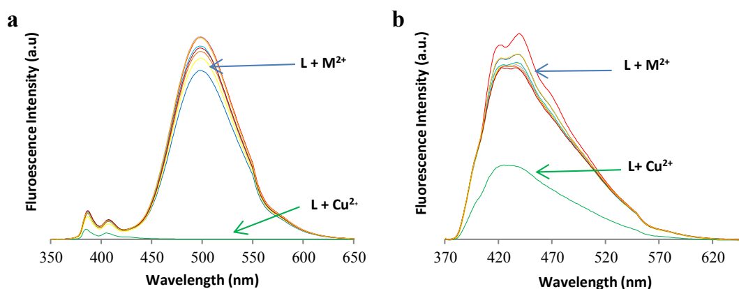
Fig. 5. Fluorescence emission spectra of L (6 \mu\text{M} , MeCN, red) upon the addition of 20 equiv of the perchlorate salts of \text{Cd}^{2+} , \text{Zn}^{2+} , \text{Ni}^{2+} , \text{Pb}^{2+} , \text{Fe}^{2+} , \text{Hg}^{2+} , \text{Co}^{2+} , \text{Cu}^{2+} ; a. PIC ( \lambda_{\text{ex}} 343 nm) and b. AIC ( \lambda_{\text{ex}} 364 nm).
