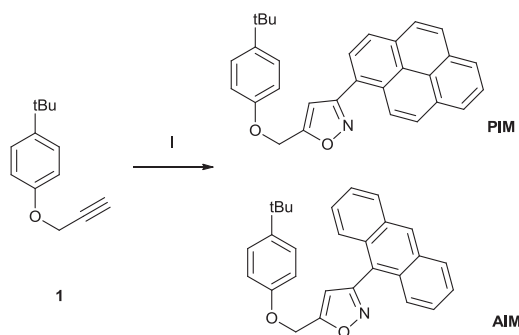
Fig. 1. Synthesis of model compounds PIM (62%) & AIM (98%): i. Chloramine-T, EtOH, reflux, 6 h, 1-pyrene carboxaldehyde oxime ( 2 ) or 9-anthracene carbaldehyde oxime ( 3 ).
