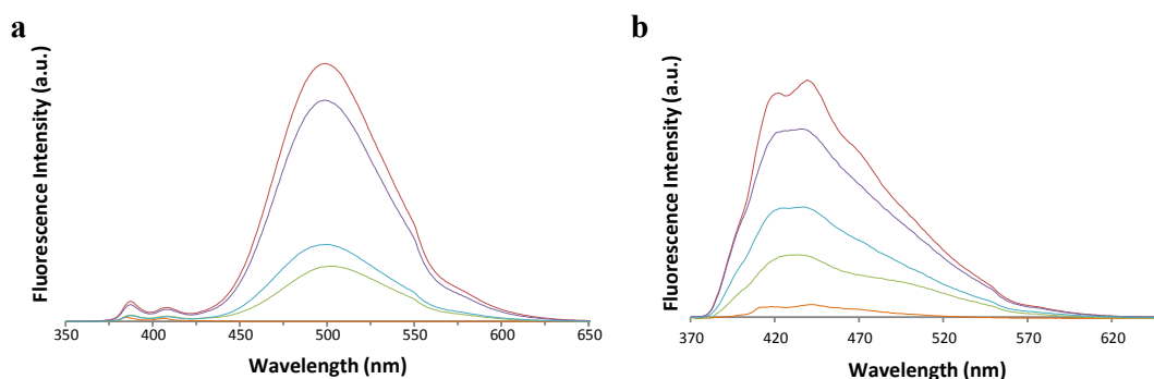
Fig. 6. Fluorescence emission spectra of L (6 \mu\text{M} , MeCN): a. PIC (red, \lambda_{\text{ex}} 343 nm) and b. AIC (red, \lambda_{\text{ex}} 364 nm) upon the addition of 100 equiv of a range of copper(II) salts: \text{Cu}(\text{ClO}_4)_2 (orange), \text{CuCl}_2 (green), \text{Cu}(\text{NO}_3)_2 (blue) and \text{Cu}(\text{CH}_3\text{CO}_2)_2 (purple).
