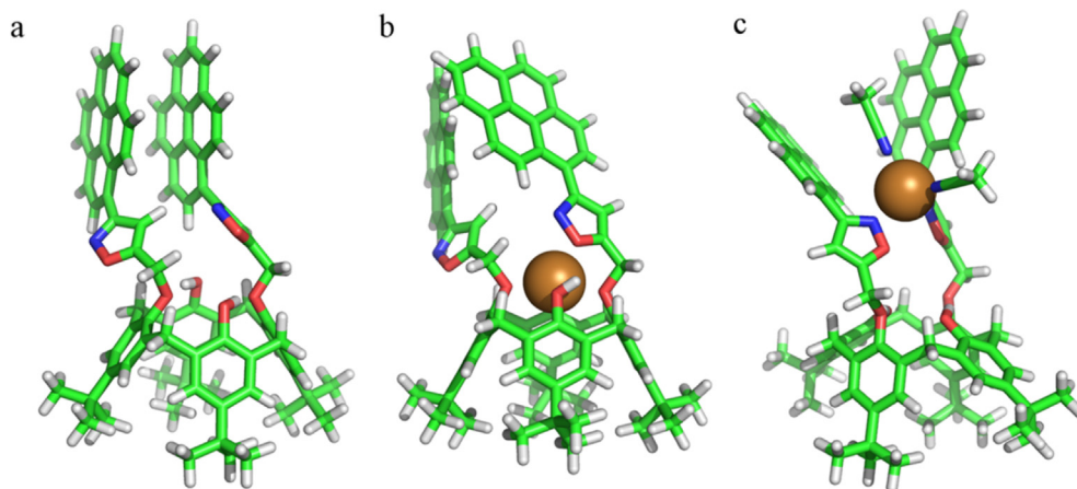
Fig. 12. Panel a: Structure of the gas-phase ground state for the unbound PIC . Panel b: Gas phase distorted square pyramidal minimum energy structure of the copper(II)/ PIC complex, Panel c: Tetrahedrally coordinated minimum energy structure of the copper(II)/ PIC in solution, where two solvent molecules complete the coordination sphere.
