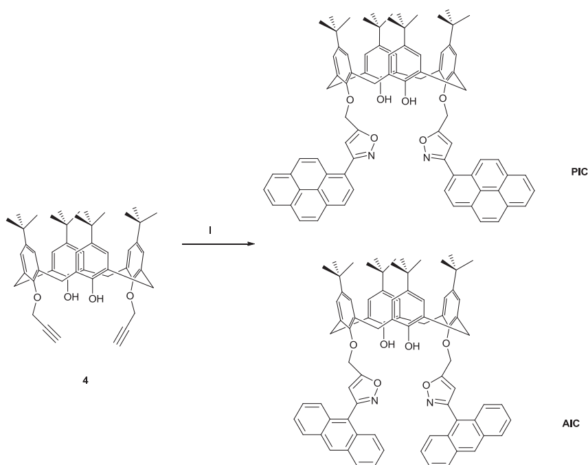
Fig. 2. Synthesis of calix[4]arene derivatives PIC (54%) & AIC (51%): i. Chloramine-T, EtOH, reflux, 1-pyrene carboxaldehyde oxime ( 2 ) or 9-anthracene carbaldehyde oxime ( 3 ), 18 h.
