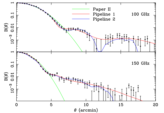
Figure 4. QUaD beam profiles at 100 GHz (top panel) and 150 GHz (bottom panel) as measured from the QSO PKS0537–441. The radial profiles as predicted using our new beam models for both pipelines are overlotted as the red and blue curves and show good agreement with the QSO data. Also shown for comparison is the elliptical Gaussian beam model used for our previous analysis in Paper II.
