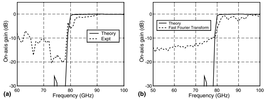
Fig. 17. (a) Measured and predicted band edge of the QUA D 100 GHz horn (NUI Maynooth) and (b) fast Fourier transform (FFT) and predicted band edge of the QUA D 100 GHz horn (Stanford University).
