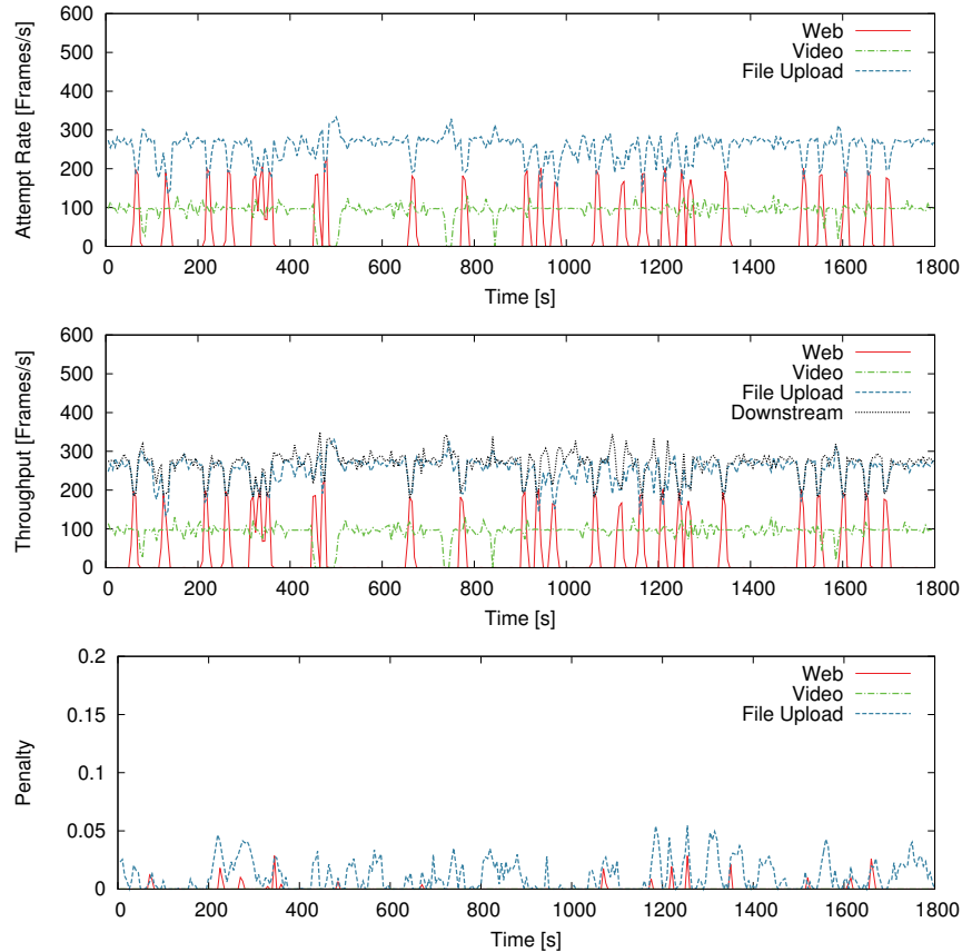
Fig. 15. WLAN consisting of four standard compliant stations generating heterogeneous traffic: file upload, web browsing, video streaming, system update (download). AP runs the proposed policing scheme. 30-minute snapshot of the attempt rate (above) and throughput (middle) attained by each flow, as well as the penalties applied by our algorithm (below). Experimental data.
