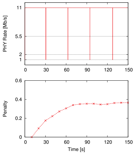
Fig. 16. WLAN consisting of three saturated stations that transmit 1,000-byte packets using the IEEE 802.11 HR/DSSS physical layer. Two stations are compliant and transmit at 11Mb/s, the third is misbehaving ( CW_{\min} halved) and runs the Minstrel RC algorithm. Clients can choose from the following set of PHY bit rates for transmission: \{1, 2, 5.5 \text{ and } 11\} Mb/s. The proposed policing scheme is executed at the AP. PHY rates selected by the selfish client (above) and penalty applied (below) over a 150s period. Experimental data.
