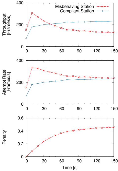
Fig. 9. WLAN consisting of three saturated stations: two compliant and one misbehaving, using a CW_{\min} half the default value. The AP runs the proposed policing scheme. Time evolution of the throughput (above), attempt rate (middle) and penalty applied by the proposed policing algorithm (below) for the misbehaving station and one fair client. Experimental data.
