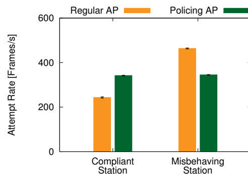
Fig. 1. Wireless network with two stations, one contending with CW_{min} = 32 (compliant) and one with CW_{min} = 16 (misbehaving). Stations always have 1,000-byte packets to send and employ the IEEE 802.11 HR/DSSS physical layer at 11Mb/s. Average and 95% confidence interval of the attempt rate attained by each station when the network operates with a regular AP, as well as with an AP running the policing scheme proposed in this paper. Experimental Data.
