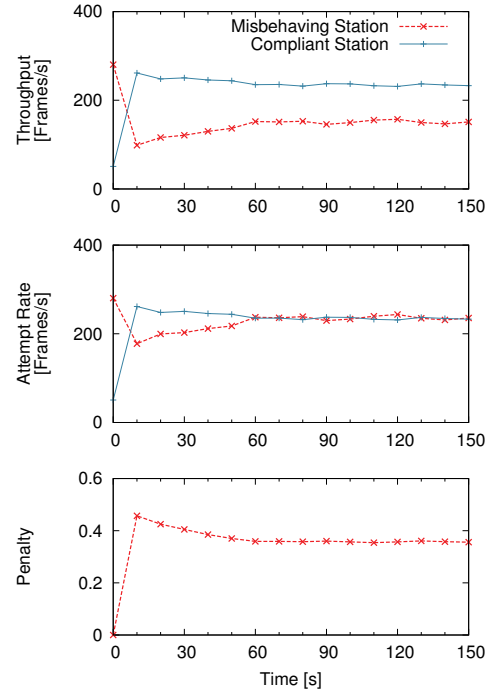
Fig. 10. WLAN consisting of three saturated stations: two compliant and one misbehaving, using TXOP = 6.413 ms. The AP runs the proposed policing scheme. Time evolution of the throughput (above), attempt rate (middle) and penalty applied by the proposed policing algorithm (below) for the misbehaving station and one fair client. Experimental data.
