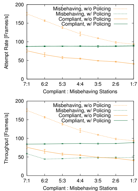
Fig. 13. WLAN consisting of eight backlogged clients transmitting 1,000-byte packets at 11Mb/s (802.11b). The ratio of compliant:misbehaving stations is varied. Selfish users contend with CW_{min} half the default value. Average and 95% confidence intervals of the attempt rate (above) and throughput (below) attained by a fair and a misbehaving station, when AP operates with and without the proposed policing scheme. Experimental data.
