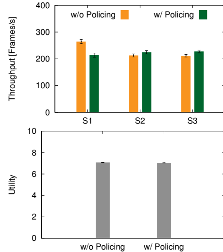
Fig. 18. WLAN consisting of three compliant stations always having 1,000-byte packets to transmit using the IEEE 802.11 HR/DSSS physical layer at 11Mb/s. Station (S1) is located next to the AP. Stations S2 and S3 are placed at a distance four times longer, thus S1 can capture the channel over S2 and S3. Average and 95% confidence interval of per-station throughput shown above with a regular AP (light bars) and an AP running the proposed policing scheme (dark bars). Network utility shown below, with and without policing. Experimental data.
