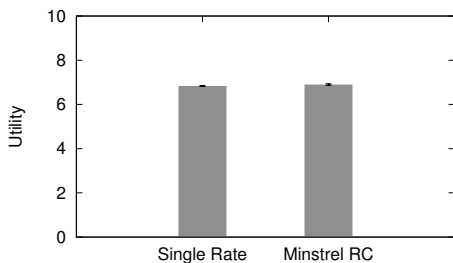
Fig. 17. WLAN consisting of three saturated stations that transmit 1,000-byte packets using the IEEE 802.11 HR/DSSS physical layer. Two stations are compliant and transmit at 11Mb/s and the third is misbehaving ( CW_{\min} halved). The proposed policing scheme is executed at the AP. Network utility when the misbehaving client runs the Minstrel RC algorithm and uses a single PHY rate for transmission respectively. Experimental data.
