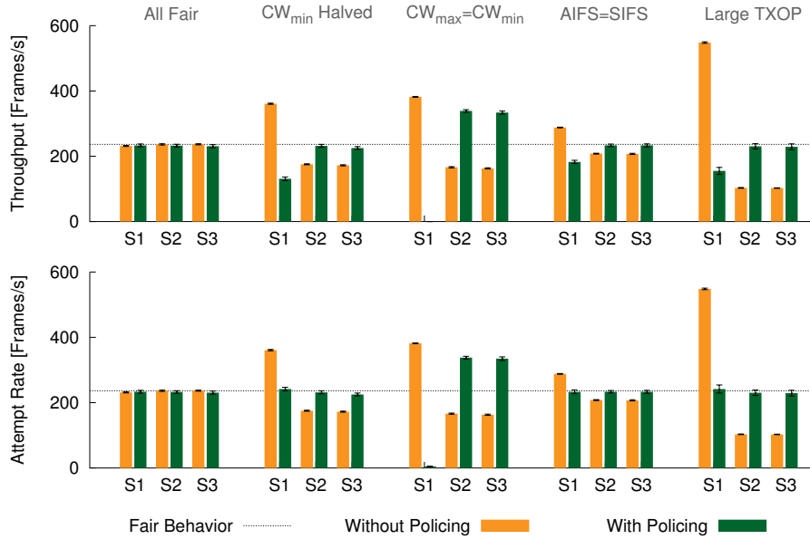
Fig. 8. WLAN consisting of three backlogged stations sending 1,000-byte packets using the IEEE 802.11 HR/DSSS physical layer at 11Mb/s. Station S1 employs one of four types of MAC misbehaviour, stations S2 and S3 are standard compliant. Average throughput (above) and attempt rate (below) of each station in each scenario, when the network operates with a regular AP (light bars) and an AP running our policing algorithm (dark bars). Also plotted is the performance of a station when all clients are fair. Experimental data.
