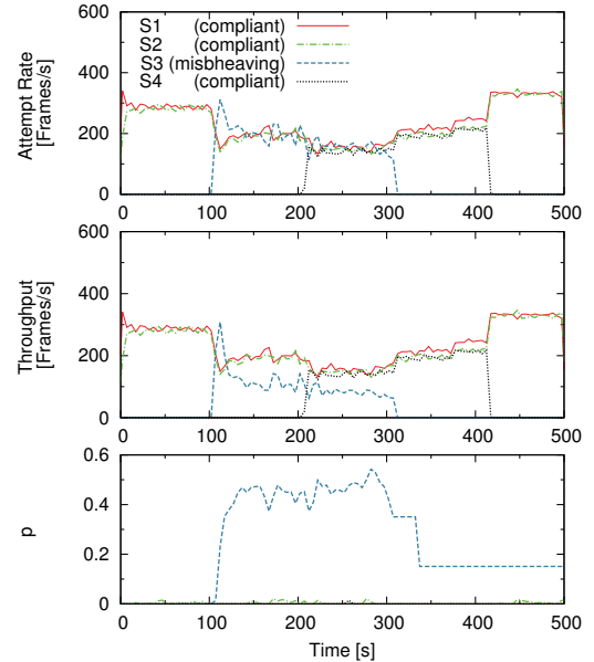
Fig. 14. WLAN with dynamic topology: two compliant stations are joined by a misbehaving one ( CW_{\min} half the default value) and subsequently by a third fair client. Stations S3 and S4 transmit for 200s each and then leave the network. The AP runs the proposed policing scheme. Time evolution of the attempt rate (above), throughput (middle) and penalty applied by the proposed policing algorithm (below) for each client. Experimental data.
