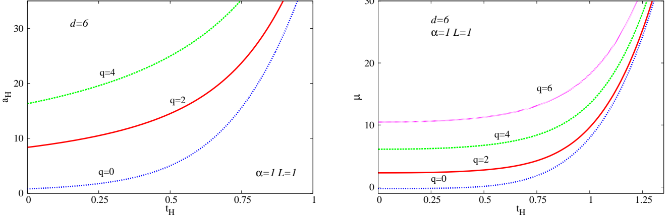
Figure 1. The reduced area a_H and mass \mu are shown as a function of reduced temperature t_H for d = 6 isotropic black branes in Einstein-Maxwell theory. Here and in Figure 3 the quantities are scaled with respect to the magnetic field on the boundary.
