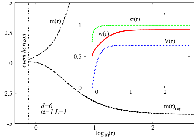
Figure 2. The profiles of a typical d = 6 Einstein–Yang–Mills isotropic black brane solution are shown as a functions of the radial coordinate r .
