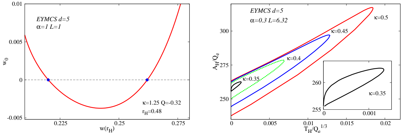
Figure 4. Left: The asymptotic value of the magnetic gauge potential w_0 is shown as a function of its value at the event horizon w(r_H) for d = 5 solutions in Einstein–Yang–Mills–Chern–Simons theory. Right: The scaled horizon area A_H is shown –for several values of \kappa – as a function of the scaled temperature T_H for d = 5 Einstein–Yang–Mills–Chern–Simons solutions with a vanishing magnetic field on the boundary.
