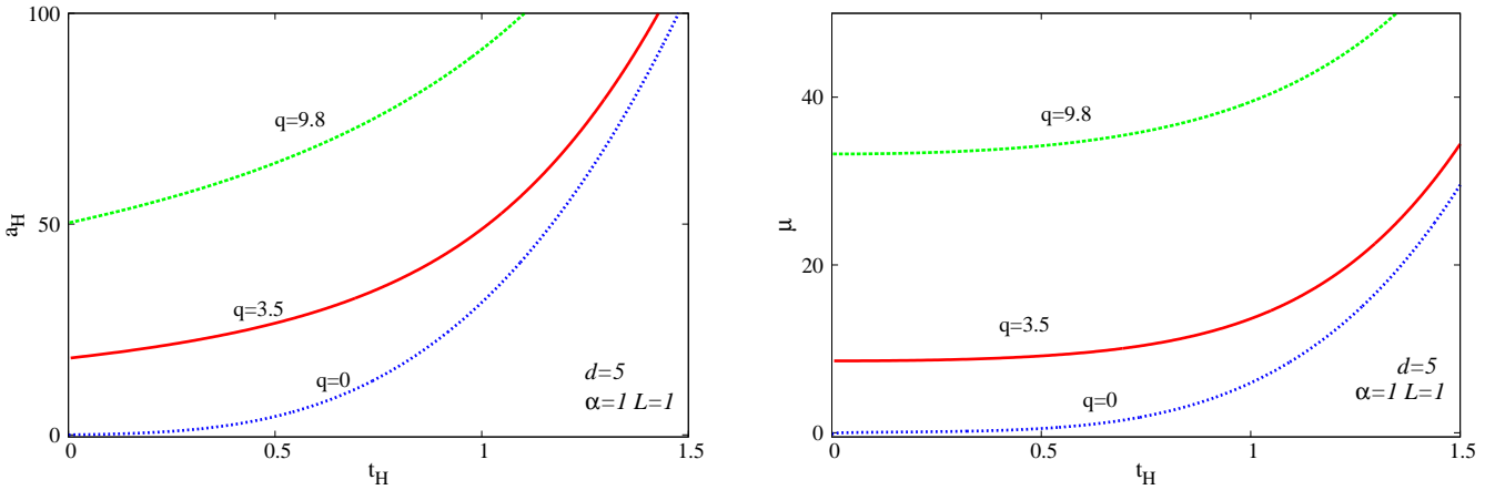
Figure 3. The reduced area a_H and mass \mu are shown as functions of the reduced temperature t_H for d = 5 isotropic black branes in Einstein–Yang–Mills theory.
