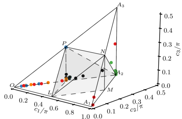
FIG. 7. (Color online) Same as Fig. 5, but control with two pulses E_J(t) and E_{JJ}(t) . Color coding as in Fig. 6.
