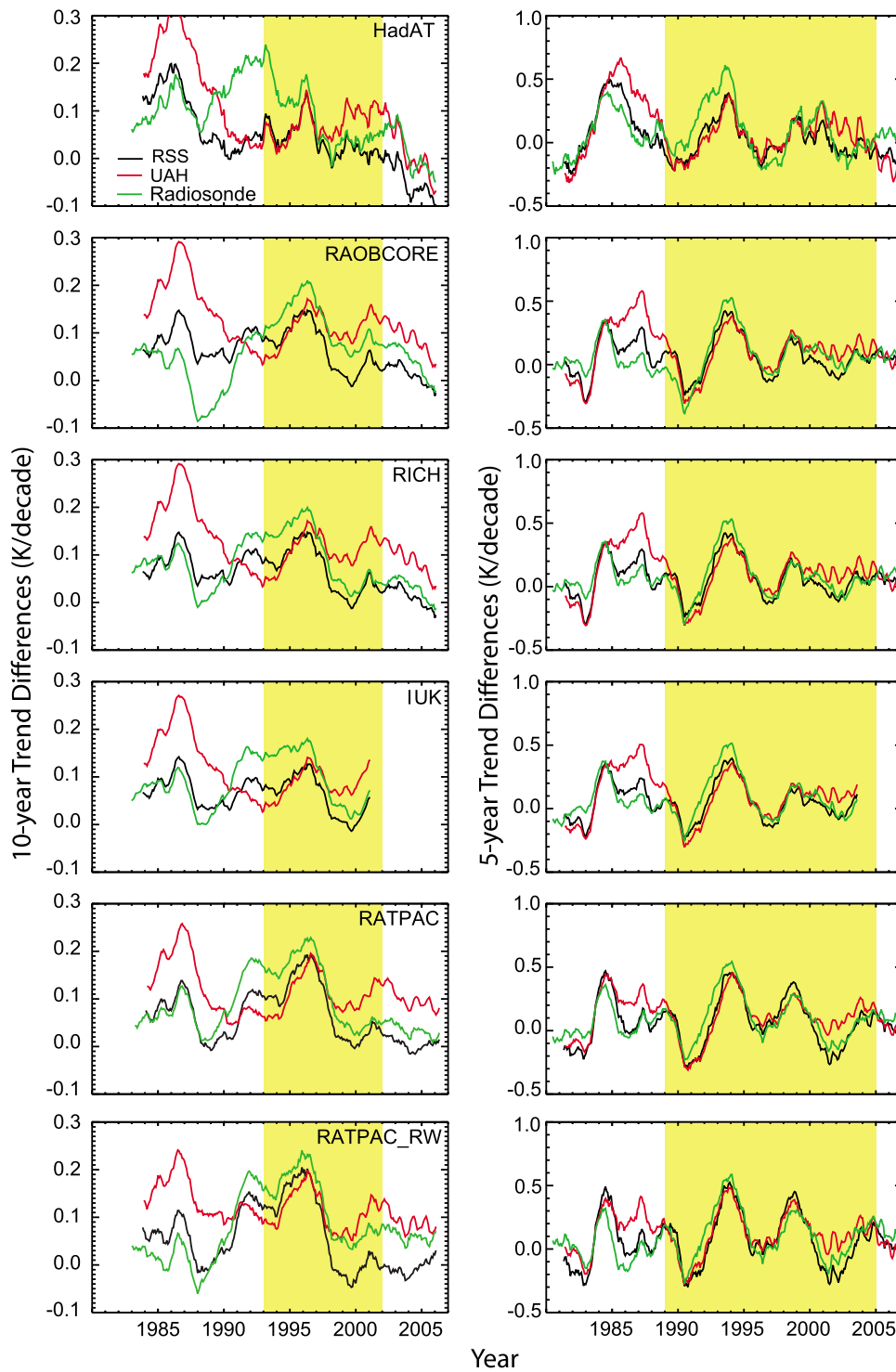
Figure 10. Differences (TLT minus TMT) in short-term trends in atmospheric temperature between adjacent layers for each radiosonde data set. In each case, the satellite data is sampled at the radiosonde locations, and the differences in spatial sampling lead to the differences between the satellite results for the different panels. The temporal range plotted in RH2008 is shaded in yellow.
