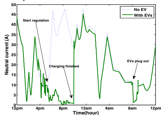
Fig. 10. Comparison of neutral current magnitude
