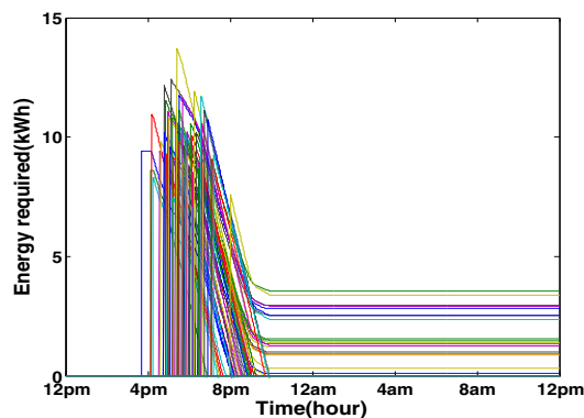
Fig. 11. Energy requirements for all EVs
