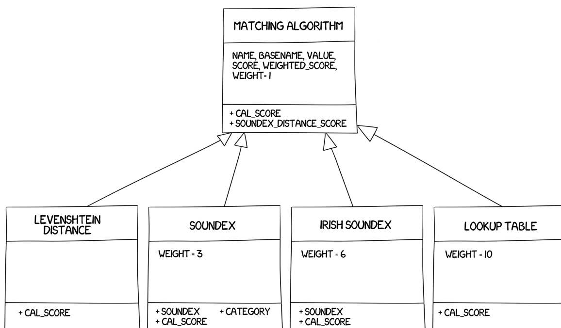
Figure 7: MatchingAlgorithm inheritance.
