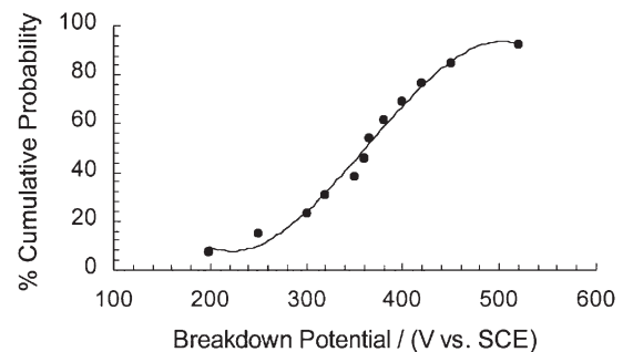
Fig. 2. Cumulative probability plot of the breakdown potentials recorded for Ti-45Ni in a 37°C phosphate buffer solution.
