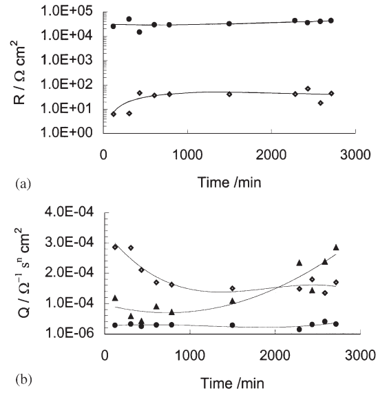
Fig. 10. (a) Resistance elements, ● R_1 , ◇ R_{pr} and (b) constant phase elements, ● Q_1 , ◇ Q_{pr} and ▲ Q_2 plotted as a function of time for Ti-45Ni in a 37°C phosphate buffer solution.
