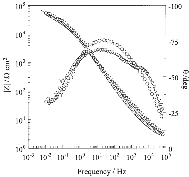
Fig. 9. Impedance data recorded for Ti-45Ni in a 37°C phosphate buffer solution; data recorded following ○ 60 min, ▽ 1000 min, — simulated data.
