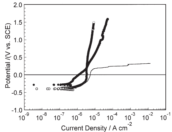
Fig. 1. Anodic polarisation plots recorded for ○ Ti, ● Ti-6Al-4V and — Ti-45Ni in a 37°C phosphate buffer solution.
