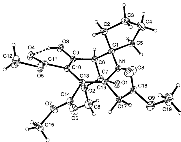
Fig. 1 X-Ray crystallographic projection of 11 .
