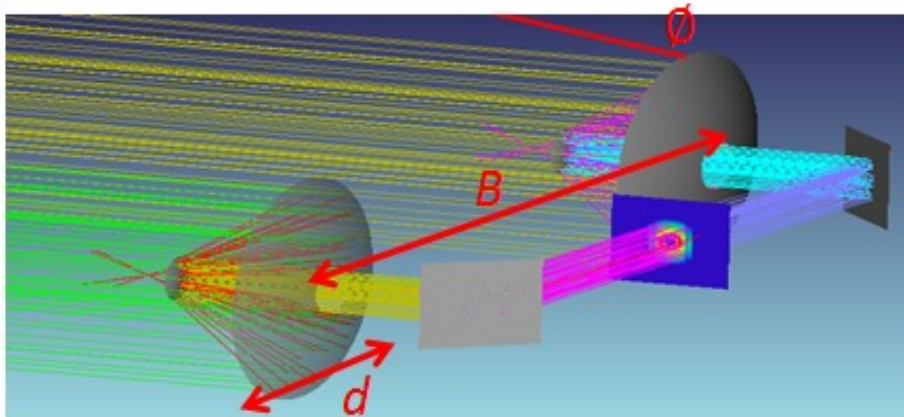
Figure 4. The two light collecting telescopes, sampling two sections of the wavefront and then redirecting the beams at 45^\circ to the central hub, represented here simply as a square. d = 2 \text{ m} , B = 2 - 50 \text{ m} , and \phi = \pm 0.5^\circ .
