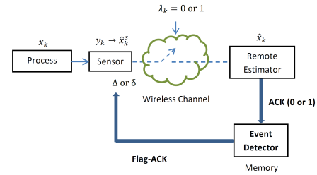
Fig. 3. System Architecture under Online Sensor Schedule.
