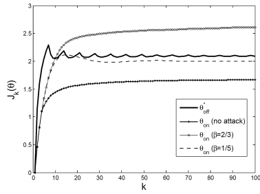
Fig. 5. Comparison between J(\theta_{\text{off}}^*) , J(\theta_{\text{on}}) and J(\tilde{\theta}_{\text{on}}) .
