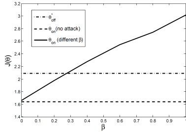
Fig. 6. Comparison of J(\tilde{\theta}_{\text{on}}) under different \beta .
