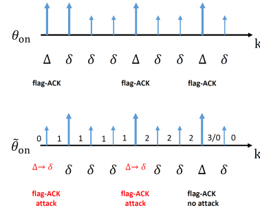
Fig. 4. Comparison between \theta_{\text{on}} and \tilde{\theta}_{\text{on}}
