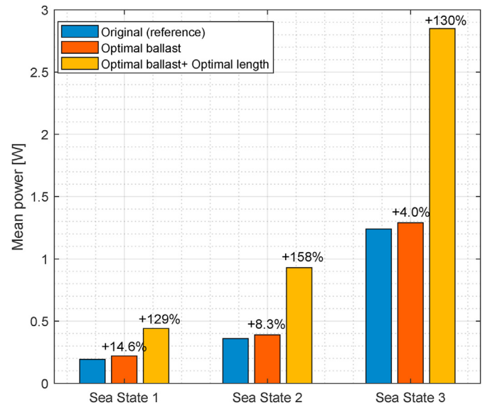
Fig. 7. Comparison of the mean power converted by the three-body hinge-barge WEC using three methods.
