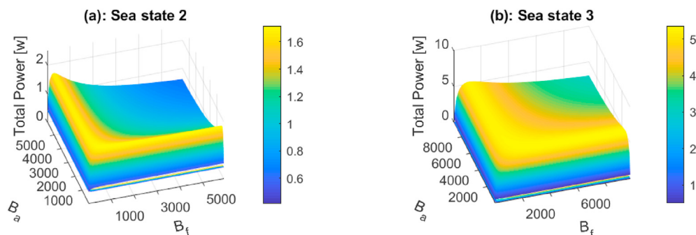
Fig. 9. Power variation of a three-body hinge-barge WEC (with control-informed ballast and geometric optimisation) over fore PTO damping coefficients ( B_f ) and aft PTO damping coefficients ( B_a ), under Sea State 2 ( H_s = 6.0\text{ cm} , T_p = 1.23\text{ s} ) and Sea state 3 ( H_s = 11.3\text{ cm} , T_p = 1.45\text{ s} ). B_f and B_a have a unit of Nms/rad . (a) Sea state 2: The device has an optimal fore barge length of 1.995 m and an optimal aft barge length of 1.08 m. (b) Sea state 3: The device has an optimal fore barge length of 1.997 m and an optimal aft barge length of 1.336 m.
