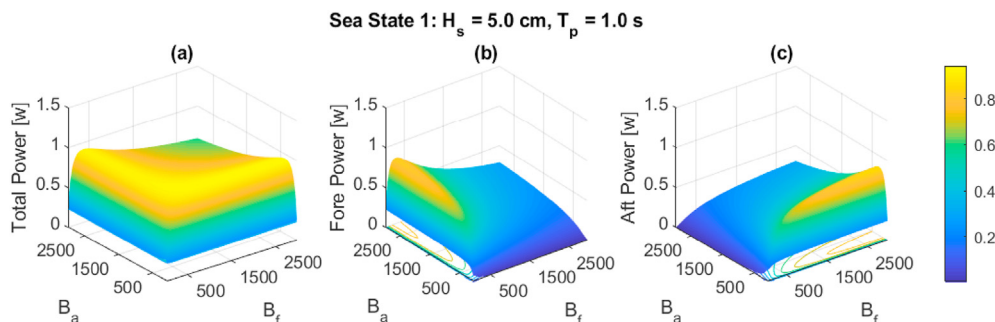
Fig. 8. Power variation of a three-body hinge-barge WEC (with control-informed ballast and geometric optimisation) over fore PTO damping coefficients ( B_f ) and aft PTO damping coefficients ( B_a ), under Sea State 1. B_f and B_a have a unit of Nms/rad . This device has an optimal fore barge length of 1.99 m and an optimal aft barge length of 1.03 m, under Sea state 1.
