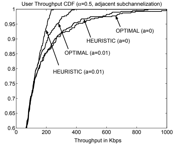
Fig. 1. Empirical CDF of users' throughputs.
