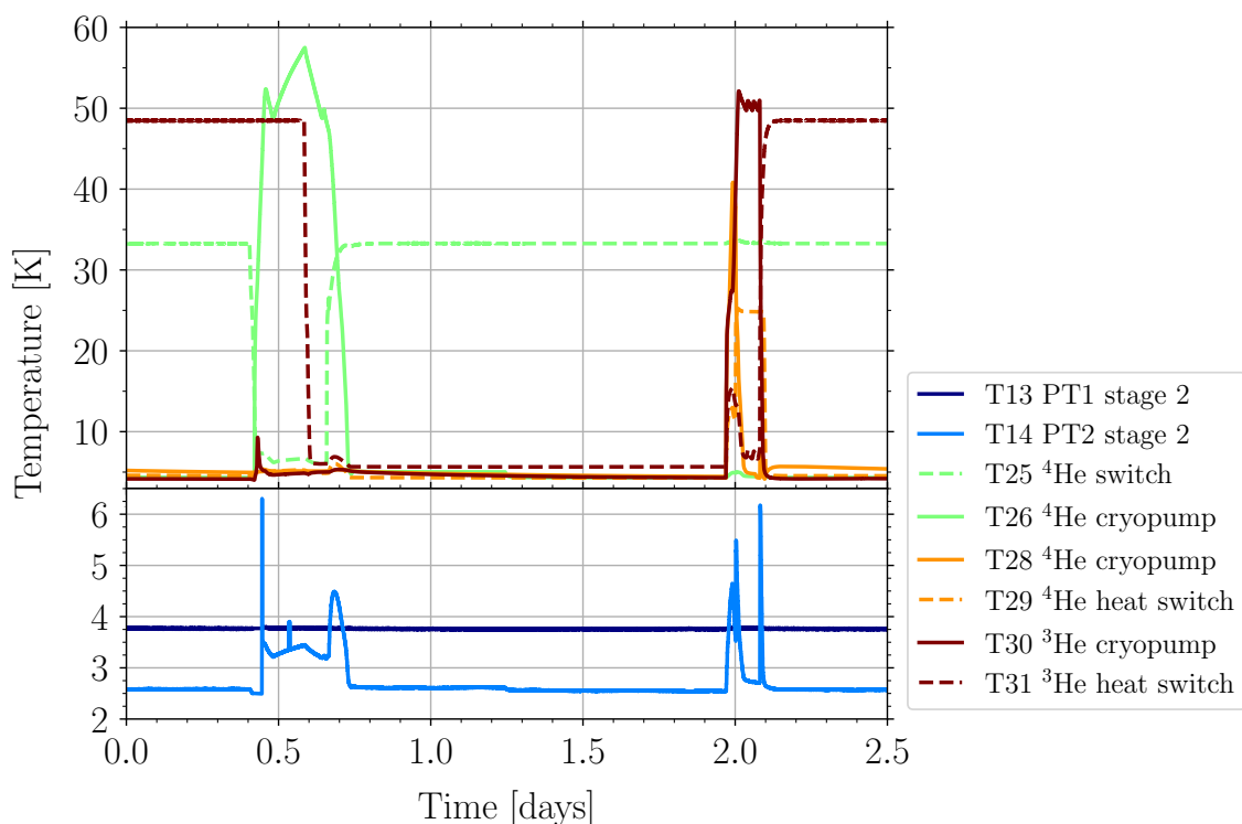
Figure 12. Temperature of the different thermometers in the 40-K and 3-K stages during sample heating cycles of the EVRs cryopumps, desorbing warm 3 He and 4 He.
