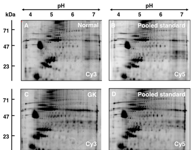
Figure 2. Comparative two-dimensional gel electrophoretic analysis of normal versus diabetic rat skeletal muscle. Shown is the 2D-DIGE analysis of the mitochondria-enriched fraction, using a pH 4-7 range in the first dimension. Individual panels represent Cy3-labelled gels of mitochondrial protein fractions from normal (A) and diabetic GK (C) skeletal muscle, as well as Cy5-labelled gels containing pooled standards (B, D). The pH-values of the first dimension gel system and molecular mass standards (in kDa) of the second dimension are indicated on the top and on the left of the panels, respectively.
