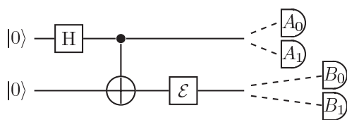
FIG. 1. A simple setup to detect nonlocality: Here, two possible measurement settings for the first (second) qubit are denoted A_i ( B_j ). When A_i and B_j are constrained to be Pauli operators, then \mathcal{E} must be a nonstabilizer operation if any Bell inequality [e.g., that given in (5)] is to be violated.
