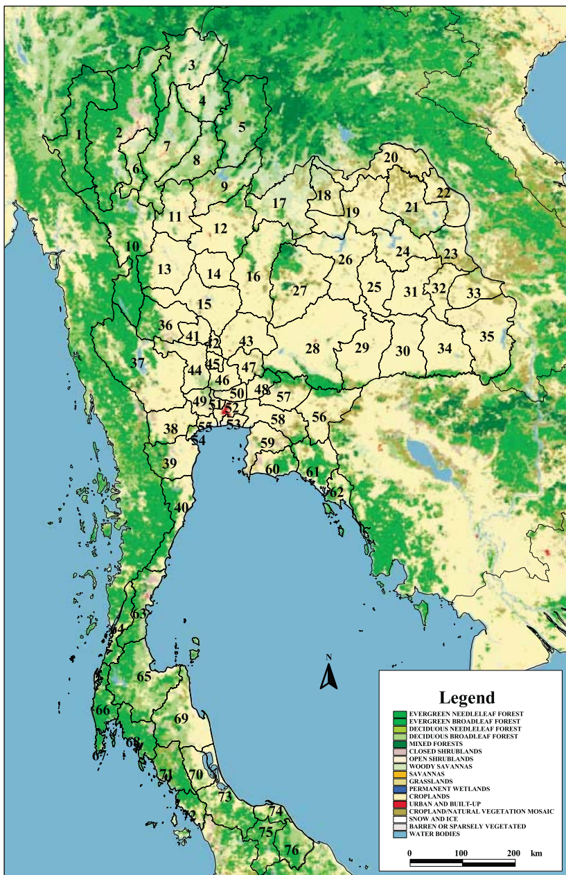
Figure 4 Map of Thailand showing vegetation type and Changwat boundaries. Changwat numbers indicated in bold.
