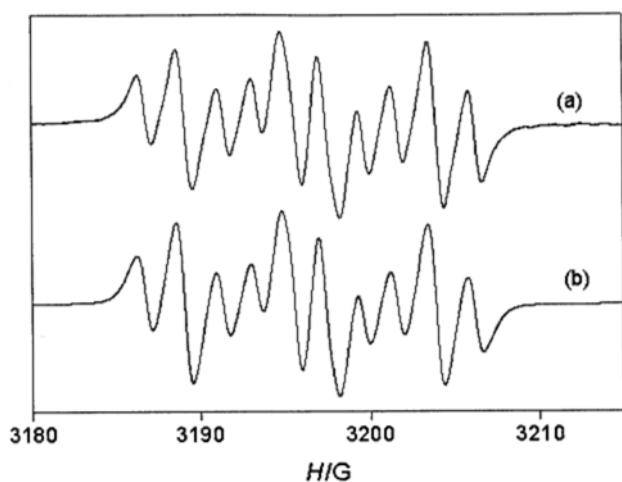
Fig. 2. (a) Epr spectrum recorded in \text{CH}_2\text{Cl}_2 at 20^\circ\text{C} of p -benzoquinone with \text{RhCl}(\text{PPh}_3)_3 ; (b) simulation of this spectrum as a doublet ( A=5.41 G) of doublets ( A=4.31 G) of triplets ( A=1.43 G).
