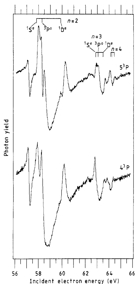
Figure 2. The excitation of the 4^3P and 5^3P singly excited states of helium as a function of the incident-electron energy. Subsequent groups of 1^1S^e , 3^1P^o and 1^1D^e autoionising states give rise to groups of structures observed in the excitation functions. The thresholds of the autoionising states in the first three groups are indicated. The 1^1S^e , 3^1P^o and 1^1D^e states in each group (indicated by the principal quantum number n=2, 3 and 4 of the outer electron) correspond to different rotational modes of the K=1 , T=0 vibrational mode in the collective rovibrational model of the doubly excited helium atom (Kellman and Herrick 1980).
