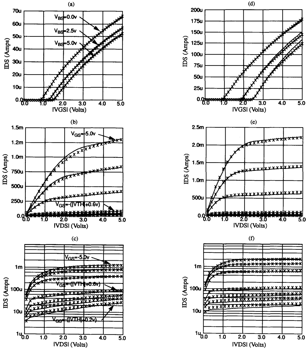
Figure 4: Measured and modeled characteristics for a 20/2μm P-channel device (a), (b) and (c) and N-channel device (d), (e) and (f). QMOS was used to extract the model parameters.
