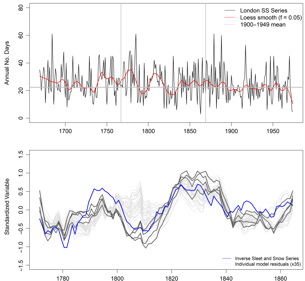
FIGURE 2 (a) Manley's Sleet and Snow Series for the greater London area 1669–1974. Also plotted is the loess smoothed ( f = 0.05 ) series. Vertical grey lines indicate years employed to investigate winter model residuals. (b) Comparison of standardized decadal mean inverse sleet and snow series (blue) 1767–1869 with standardized decadal mean model residuals. Grey lines represent median residuals from each model, dark grey lines are models based on observations only. Black line shows the ensemble median residual
