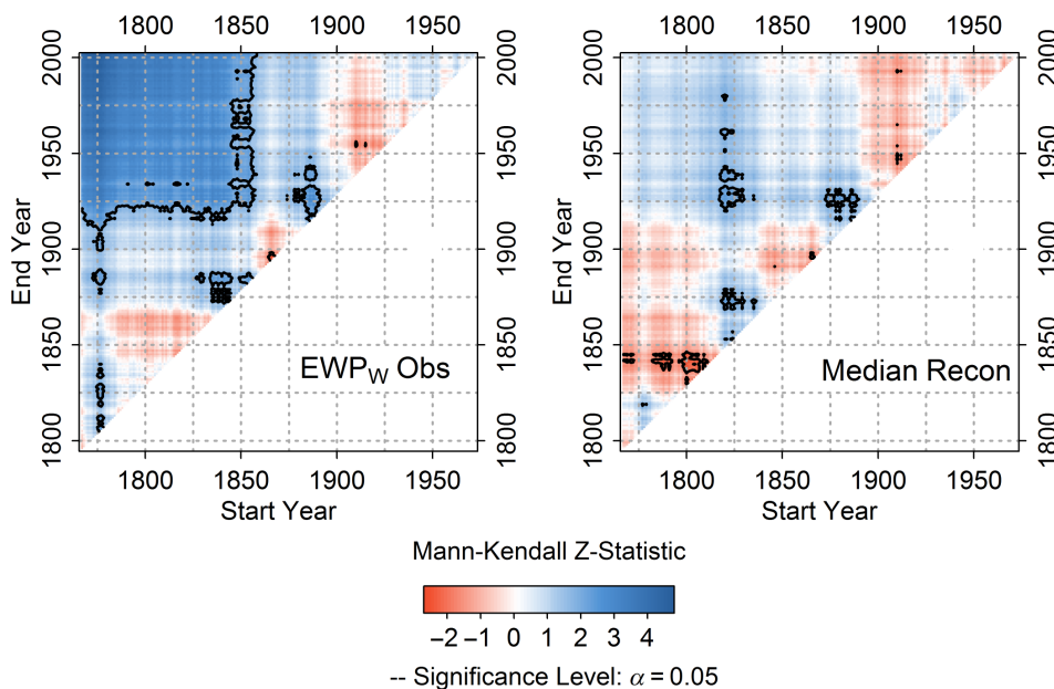
FIGURE 3 Mann Kendall Zs scores for observed EWP_w and median model reconstruction for all combination of start and end years (minimum 30-years) for the period 1767–2002. Black contour marks significant trends ( p < .05 )
