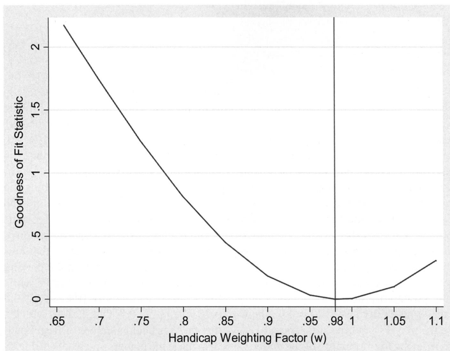
Figure 1. Measure of fairness across alternative handicap systems.
