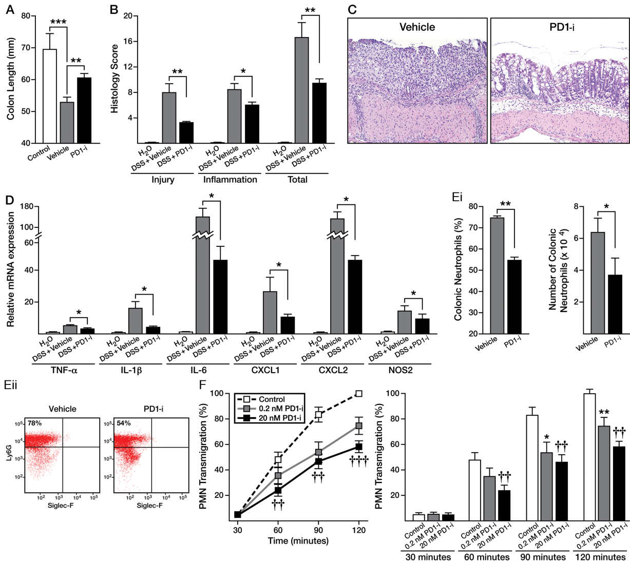
Figure 8 Protectin D1 (PD1)-isomer (PD1-i) treatment attenuates colitis in PHIL -mice via attenuation of neutrophil migration. PHIL -dextran sodium sulfate (DSS)-colitis mice were treated with PD1-isomer or vehicle via intraperitoneal injection 0.05 mg/kg daily throughout the course of colitis which lasted 6 days. Upon sacrifice, colons were excised and (A) colon length measured. (B) Injury, inflammatory and total histology scores were assessed and (C) representative H&E-stained sections from PHIL -DSS-mice treated with PD1-isomer or vehicle (100 \times magnification). (D) Proinflammatory cytokine and neutrophil-associated chemokine mRNA production was examined in PD1-isomer versus vehicle-treated PHIL -DSS-mice. (E and F) Flow cytometric analysis of lamina propria infiltrates for neutrophil percent and absolute number comparing PD1-isomer with vehicle-treated PHIL -DSS-controls. Data are expressed as means \pm SEM of 3–7 individual mice per group, and represent 2 independent experimental repeats. (G) In vitro examination of the effects of PD1-isomer on Formyl-Methionyl-Leucyl-Phenylalanine-induced neutrophil-colon epithelial monolayer (Caco-2) transmigration; dose-dependence and time-dependence. Data are expressed as means \pm SEM of three individual donors and three independent experimental repeats. * p < 0.05, ** p < 0.01 0.2 nM PD1 versus controls. † p < 0.01, †† p < 0.001 20 nM PD1-isomer versus controls.
