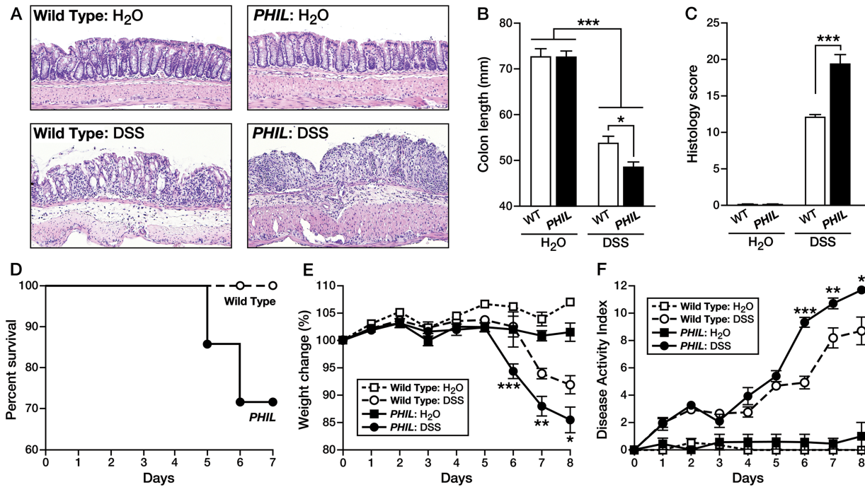
Figure 2 Protective role for eosinophils in acute colitis. Dextran sodium sulfate (DSS) or water-vehicle was administered to wild type (WT)-mice and PHIL -mice. (A) Representative H&E-stained sections of colons from WT-DSS and PHIL -DSS mice (100× magnification), (B) Colon lengths were assessed upon sacrifice and (C) A histological scoring tool combining injury and inflammation was applied to H&E-stained sections following 6 days of colitis. (D) Kaplan–meier survival curve comparing PHIL -DSS and WT-DSS littermates. (E) Colitis-induced weight loss as a percentage of day zero and (F) overall disease activity index calculated in PHIL compared with WT controls following 8 days of colitis. Data are expressed as means±SEM of 15 individual control mice and seven individual mice per DSS group and represent >3-independent experimental repeats. * p < 0.05 , ** p < 0.01 , *** p < 0.001 .
