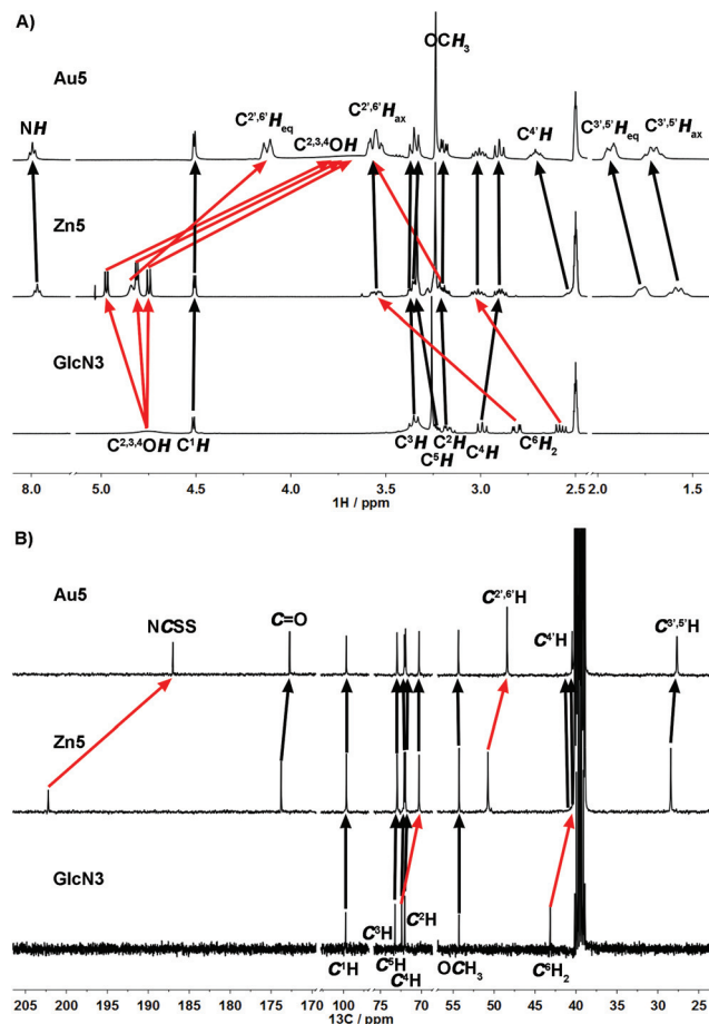
Fig. 4 Comparison of the ^1\text{H} (A) and ^{13}\text{C}(^1\text{H}) (B) NMR spectra in \text{DMSO-}D_6 of 1-O-methyl-6-amino-6-deoxy- \alpha -D-glucopyranoside (GlcN3), [\text{Zn}^{\text{II}}(\text{SSC-Inp-GlcN3})_2] (Zn5) and [\text{Au}^{\text{III}}\text{Br}_2(\text{SSC-Inp-GlcN3})] (Au5).
