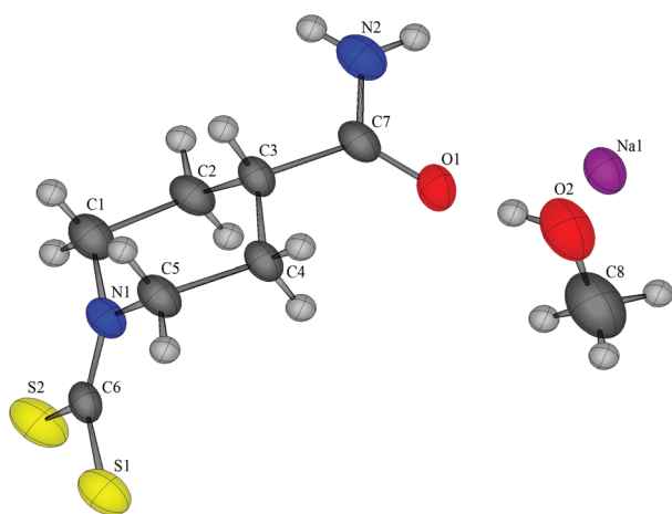
Fig. 1 X-ray crystal structure with atom numbering scheme for Na(SSC-Inp-NH 2 ) (CCDC 1835869 † ) (50% displacement ellipsoids).
