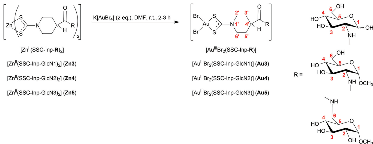
Scheme 5 Synthesis of the gold(III)-dithiocarbamate glycoconjugates via transmetalation.
