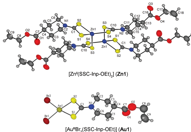
Fig. 3 X-ray crystal structure with atom numbering scheme for Zn1 (CCDC 1835870†) and Au1 (CCDC 1835871†) (50% displacement ellipsoids).
