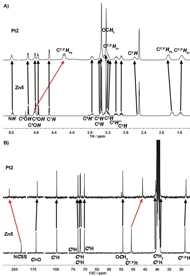
Fig. 5 Comparison of the ^1\text{H} (A) and ^{13}\text{C}(^1\text{H}) (B) NMR spectra in \text{DMSO-}D_6 of [\text{Zn}^{\text{II}}(\text{SSC-Inp-GlcN3})_2] (Zn5) and [\text{Pt}^{\text{II}}(\text{SSC-Inp-GlcN3})_2] (Pt2).
