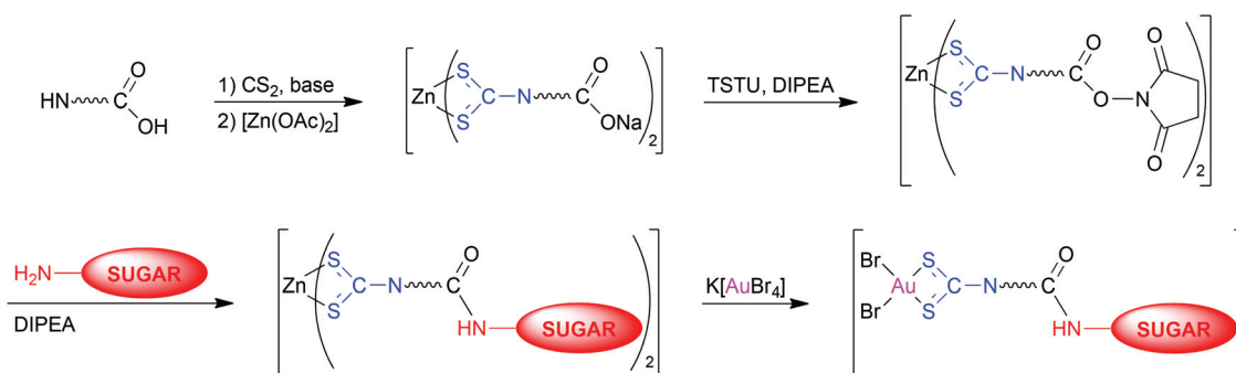
Scheme 1 General synthetic route to gold(III)-dithiocarbamate glycoconjugates.
