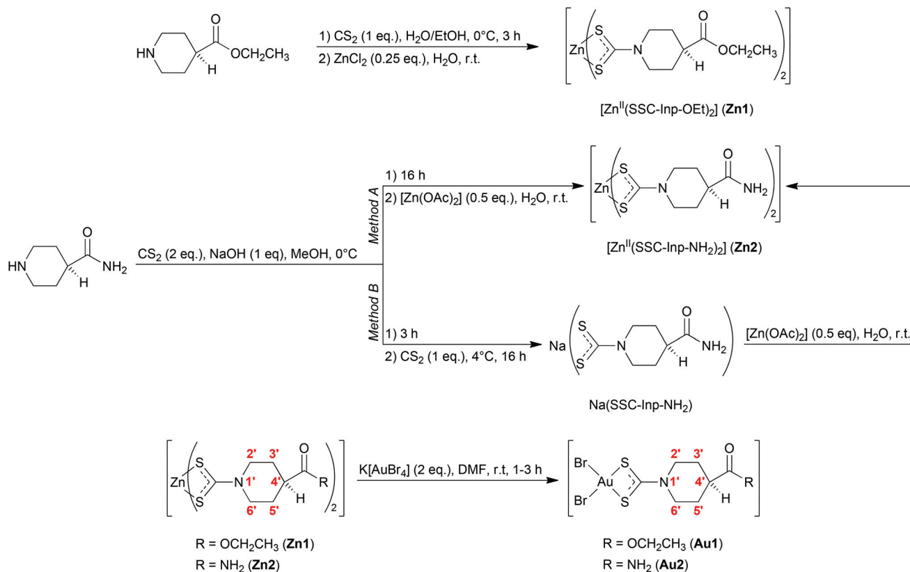
Scheme 3 Synthesis of the model ( i.e. non-glycosylated) gold(III)-dithiocarbamate derivatives via transmetalation.
