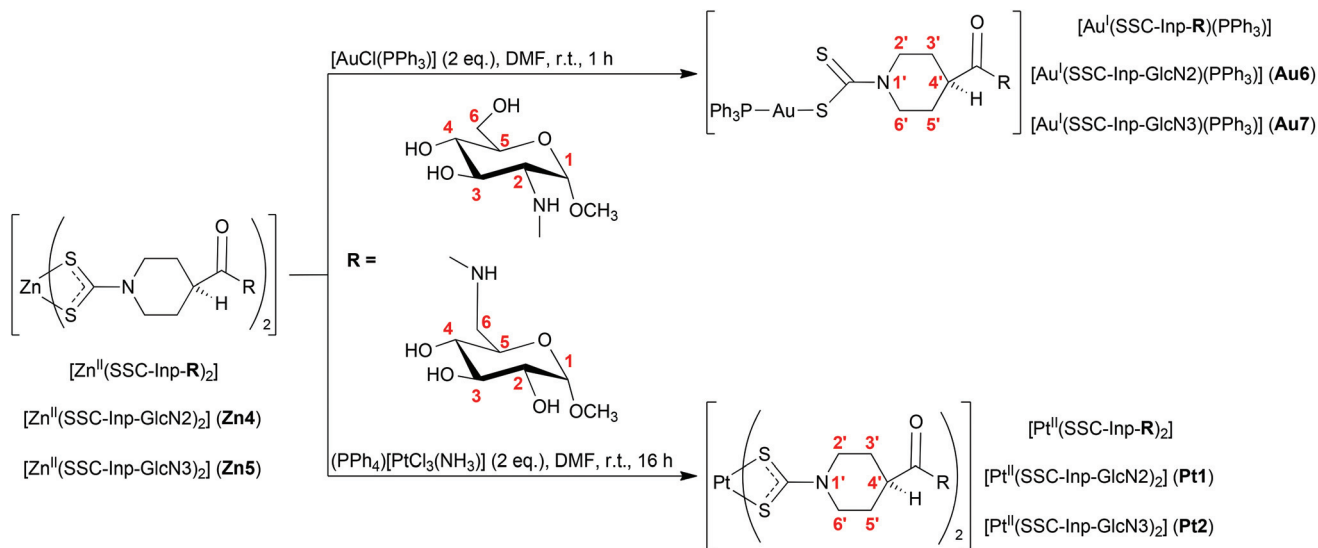
Scheme 6 Synthesis of the gold(I)- and platinum(II)-dithiocarbamato glycoconjugates via transmetalation.
