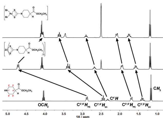
Fig. 2 Comparison of the ^1\text{H} NMR spectra in \text{DMSO-}d_6 of ethyl isonipecotate, [\text{Zn}^{\text{II}}(\text{SSC-Inp-OEt})_2] ( Zn1 ) and [\text{Au}^{\text{III}}\text{Br}_2(\text{SSC-Inp-OEt})] ( Au1 ).
