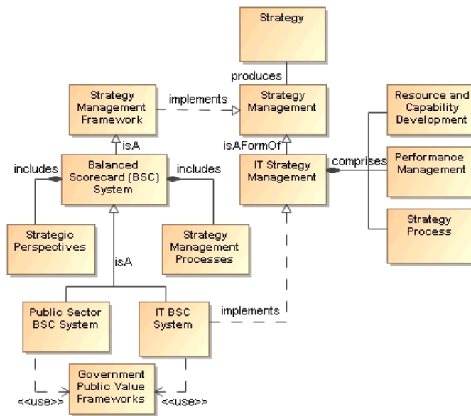
Figure 1: Conceptual Model for ITSM
