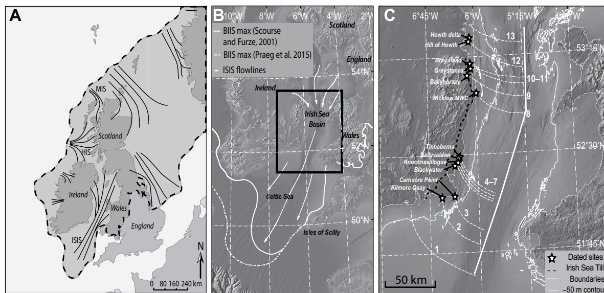
Figure 1. (A and B) Location map of study area within former British–Irish Ice Sheet (BIIS) and (A) a close up of its relative position with respect to the southern portion of the former BIIS. (C) Study area with solid white line indicating trough axis used to calculate axial retreat distances. Dashed white lines are boundaries defined in Bayesian sequence model, numbered as in Figure 2 and Table 5. Note Boundary 9 is constrained by samples from altitude, hence its location within the sequence. Sample locations are shown with white stars and site names are as Tables 1 and 5. The thick black line denotes the limit of till-bearing accessory erratics indicative of an Irish Sea provenance. MIS—Minch Ice Stream; HIS—Hebrides Ice Stream; ISIS—Irish Sea Ice Stream; MWC—meltwater channel.
