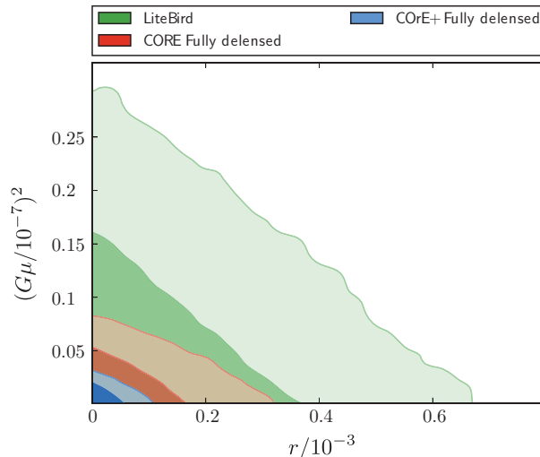
Figure 38: Likelihood contours of the r-(G\mu)^2 posterior for models with both tensors and defects (cosmic strings), marginalized over all other parameters, for LiteBIRD, CORE, and CORe+. The CORE and CORe+ contours are given for the fully delensed case, representing the best possible constraints attainable, while LiteBIRD contours are given for the standard case. In all cases light shading represents 1\sigma and dark shading 2\sigma . For comparison, the current Planck marginalized 95% confidence limits on these models are (G\mu/10^{-7})^2 < 3.4 ( f_{10} < 0.011 ) and r < 0.11 .
