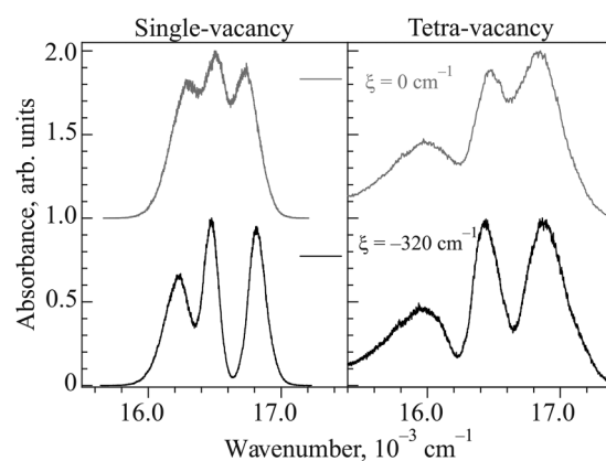
FIG. 3. Simulated spectra generated at T = 50 K when neglecting (top traces) and including (bottom traces) the spin-orbit Hamiltonian into the description of the interaction between atomic sodium and the surrounding xenon atoms. The panel on the left shows the results for the SV site of Na/Xe—that on the right shows the results for the TV site. The magnitude of the spin-orbit coupling used was -320 cm -1 which is the value determined in the matrix MCD study of Na/Xe presented in Ref. 4.
