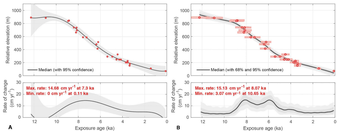
Fig. 6. Example output from estimating continuous deglaciation rates using the A) Fourier and B) spline models. The upper panel is the modelled profile for an example vertical transect (Scott and Reedy Glaciers, Antarctica; Spector et al., 2017). The mean exposure ages are also plotted, with rectangles representing the age and elevation uncertainties used in the spline-based regression. The lower panel is the corresponding rate of change. Maximum and minimum rates, and their respective timings, are also computed.
