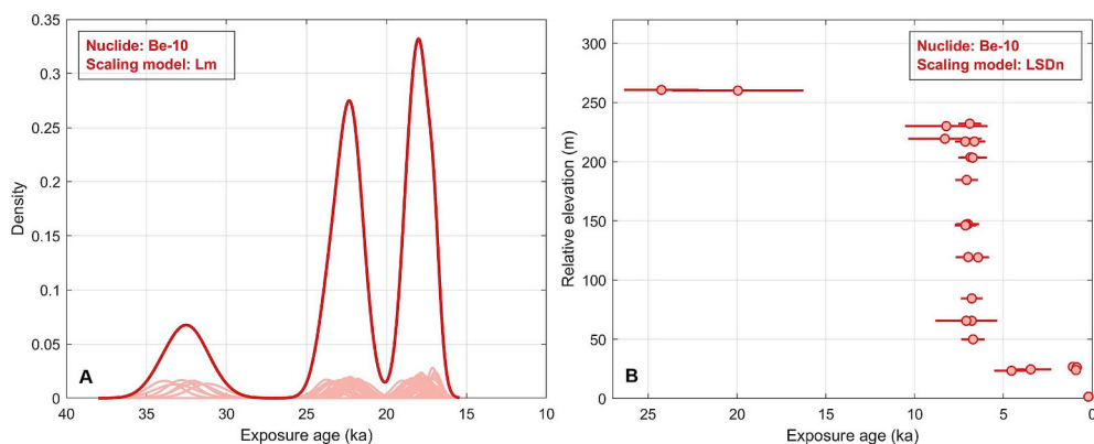
Fig. 3. Exposure ages plotted as A) kernel density estimates for samples from a sequence of moraines (Ohau II–VI, Lake Ohau, New Zealand; Putnam et al., 2013), and B) a vertical transect recording ice sheet surface lowering (Mt Suess and Low Ridge, Mackay Glacier, Antarctica; Jones et al., 2015). These are examples of the plotted outputs from the tools ‘Calculate ages’ and ‘Plot ages’, which are able to highlight temporal and spatial patterns within datasets.
