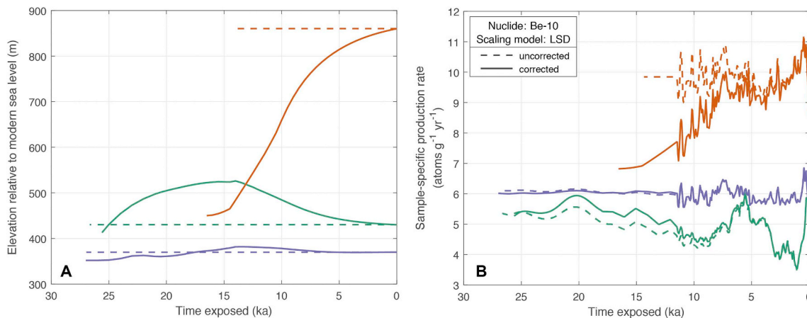
Fig. 8. Effects from GIA. A) The elevation of a sample site relative to present since first exposed, and B) the corresponding change in the site-specific production rate through time. The dashed line assumes no change in GIA, while the solid line is corrected for GIA effects. The orange site is in a region of substantial glacial isostatic uplift (central Norway), the green site was previously isostatically elevated at a ‘peripheral bulge’ (north-eastern USA), and the purple site is from a region of minor past surface elevation change (central England). The examples were generated using the ICE-6G ice model and LSD nuclide scaling model. The high-frequency production rate variability during the last ~12 ka is from changes in the solar output; the scaling model uses an average value prior to this time as any variability is undefined (Lifton et al., 2014).
