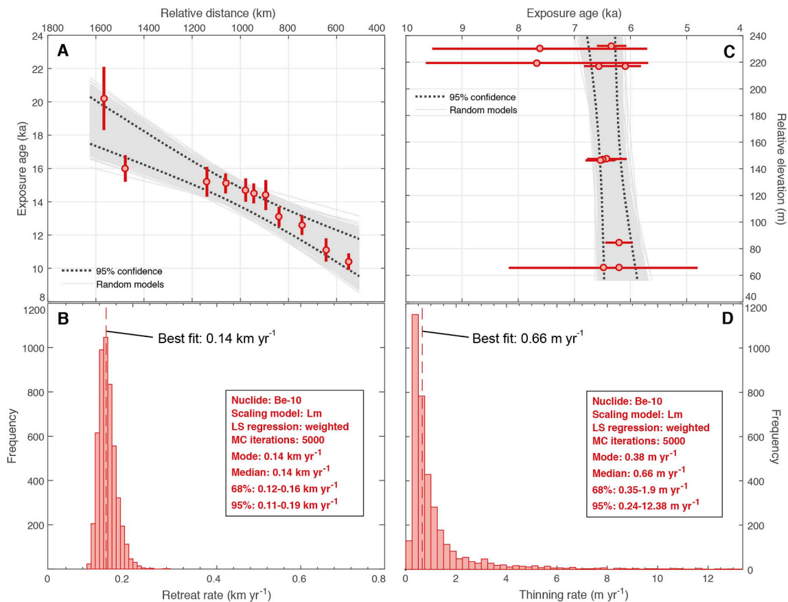
Fig. 5. Example outputs from estimating average deglaciation rates using the linear model. A) The individual linear regressions (grey lines) and the 95% confidence bounds (dashed black lines) are shown for a Monte Carlo (MC) least-squares (LS) linear regression analysis on a horizontal transect of exposure ages. The example data is from the ‘Sweden’ transect of Cuzzone et al. (2016) and references therein (using the weighted mean ages from individual sites). B) A histogram showing the corresponding distribution of retreat rates produced by each iteration of the linear regression analysis. C) and D) are the same as A and B, but for a vertical transect of exposure ages from Mackay Glacier, Antarctica (Jones et al., 2015).
