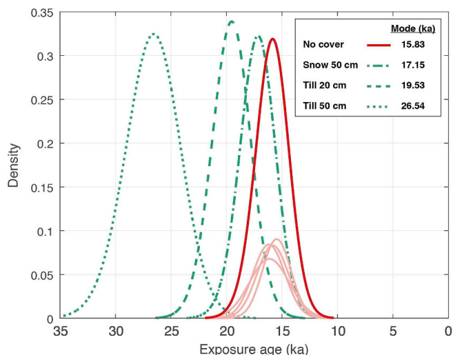
Fig. 7. Effects on exposure ages from example scenarios of material covering sampled rock surfaces. The raw, uncorrected exposure ages are shown as kernel density estimates in light red with the summed density estimate of the dataset as a dark red line. The green curves represent the summed density estimates for varying degrees of shielding by overlying materials (individual age distributions are not shown for clarity), calculated using the ‘Correct for surface cover’ tool. The dot-dashed curve is cover by 50 cm of snow (assumed density of 0.27 \text{ g cm}^{-3} ), the dashed curve is cover by 20 cm of till (assumed density of 1.8 \text{ g cm}^{-3} ), and dotted curve is cover by 50 cm of till. The greater the thickness and density of cover material, the larger the age correction.
