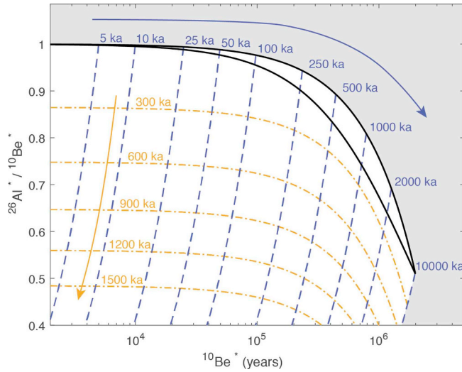
Fig. 1. A two-isotope diagram for normalised ^{10}\text{Be} and ^{26}\text{Al} concentrations. During continuous exposure, the ^{10}\text{Be} concentration increases until it becomes saturated and is at secular equilibrium (upper black line). Meanwhile, the ^{26}\text{Al}/^{10}\text{Be} ratio decreases. Surfaces that are continuously exposed but that undergo different degrees of constant erosion follow diverging trajectories until saturation is reached (lower black line). Any rock surfaces with measured concentrations that fall between these lines – the simple exposure region – are assumed to have been continuously exposed with a “simple” exposure history. Concentrations that plot above these lines (in the grey area) are either not feasible and imply issues with the geochemistry or measurement of a sample, imply that a sample was once exposed at a higher elevation (larger production rate) and then transported to a lower elevation, or indicate that a sample underwent production for a substantially long period at depth (larger ^{26}\text{Al}/^{10}\text{Be} production ratio) before arriving at the surface. Concentrations that plot below the simple exposure region indicate that the sampled surface has been buried with a “complex” exposure history. Isochrones highlight points of equal exposure time (purple dashed lines) and burial time (orange dot-dashed lines).
