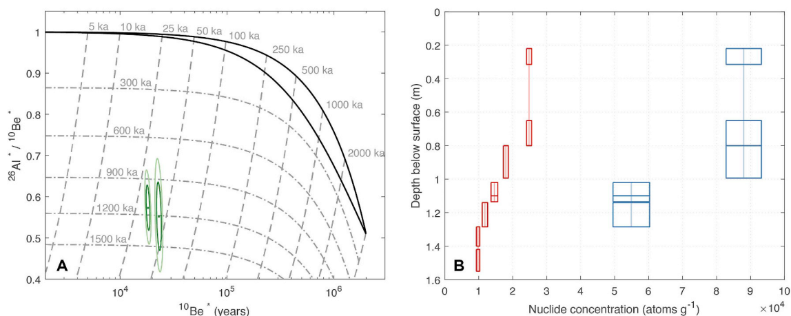
Fig. 2. Nuclide concentrations plotted A) on a two-isotope diagram (at 1 and 2 sigma), and B) as a function of depth (at 1 sigma). These are examples produced by the tool ‘Plot isotope concentrations’, which reproduce previously published plots of ^{10}\text{Be} (red) and ^{26}\text{Al} (blue) nuclide concentrations that were measured in a bedrock core (Schaefer et al., 2016). In this case, those core segments that were combined for nuclide measurement are automatically detected based on common sample depths (linked with a vertical line through the means in B) in order to produce the equivalent ^{10}\text{Be} and ^{26}\text{Al} nuclide concentrations that are shown in A. It is unlikely that samples would be combined for surface rock samples, and therefore each sample would be plotted on the two-isotope diagram separately.
