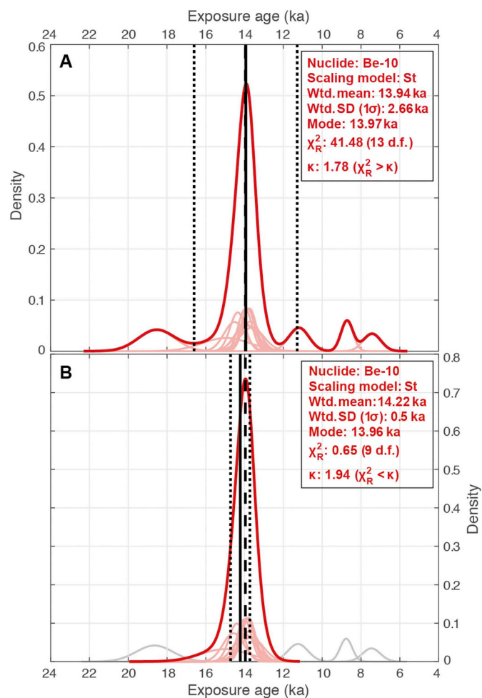
Fig. 4. Exposure ages from a moraine plotted as kernel density estimates A) for the initial raw dataset, and B) following the removal of outliers. The example dataset is from Torres del Paine, southern Patagonia (TDPIII, n = 14 ; García et al., 2012). Using the ‘Calculate ages’ or ‘Plot ages’ tool, the probability distribution of each sample is plotted in light red and the summed distribution of the dataset is plotted as a bold red line. Additionally, the mode (black dashed line), weighted mean (black solid line) and weighted standard deviation (SD; black dotted lines) of the dataset are shown, and the reduced chi-squared ( \chi^2_R ) and associated criterion ( \kappa ) are calculated; if \chi^2_R < \kappa then there is a > 95% probability that the data represent a single population (d.f. is degrees of freedom). Four outliers were identified (plotted in grey) and removed in this example using a generalised extreme Studentized deviate (gESD) test with the ‘Remove outliers’ tool.
