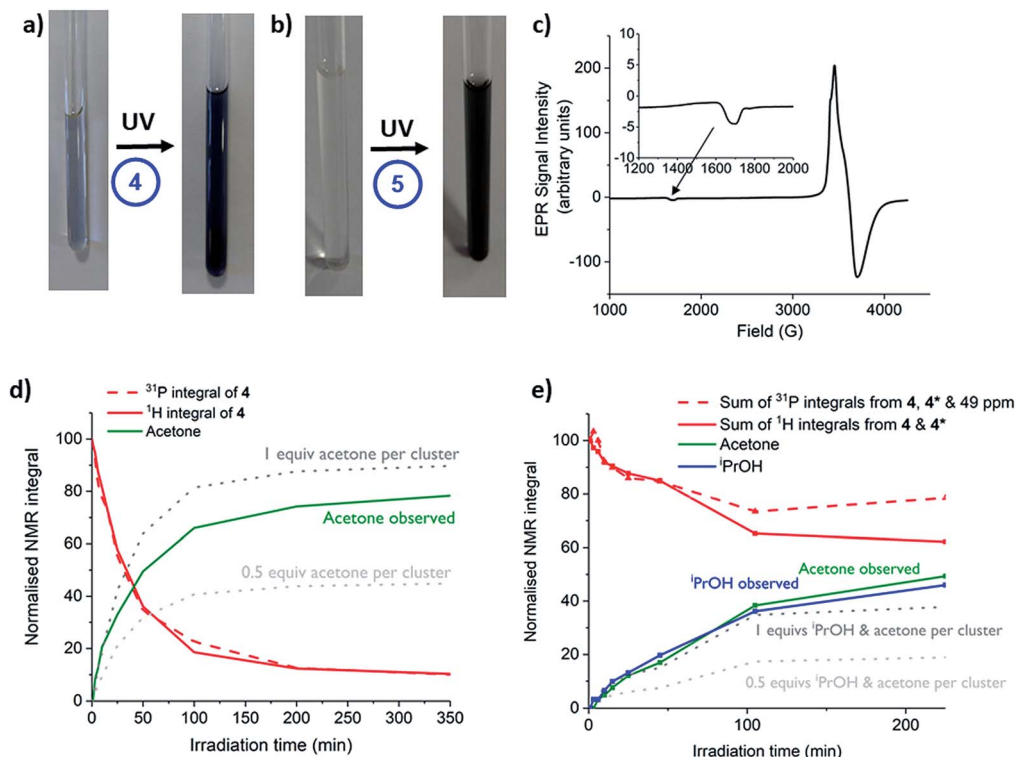
Fig. 5 (a and b) Photographs of toluene solutions of 4 and 5 (with 30 equiv. 1 PrOH) before and after irradiation (a), 13 h, MW-UV; (b), 3 h, LW-UV. (c) X-band EPR spectrum at 10 K of 4 after photo-reduction with MW-UV (7.5 h, [4] = 10 mM, 9 : 1 toluene : 1 PrOH) with small signal at ~1700 G enhanced. (d and e) Normalised NMR integrals of 4, acetone and 1 PrOH during MW-UV irradiation in toluene ((d): 30 equiv. 1 PrOH; (e): 30 equiv. pyridine), dotted lines show the expected amount of acetone that will be produced by a 1-electron redox process (0.5 equiv. per cluster) or a 2-electron redox process (1 equiv. per cluster), estimated from the consumption of 1 H integrals of 4. N.B. 4* and the 31 P signal at 49 ppm remain uncharacterised.
