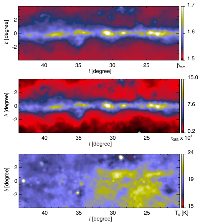
Fig. 8. Maps of the dust parameters. Top: \beta_{\text{mm}} , which results from the best linear fit to the correlation with optical depth given by Eq. (2); middle: \tau_{353} ; bottom: T_{\text{d}} .
