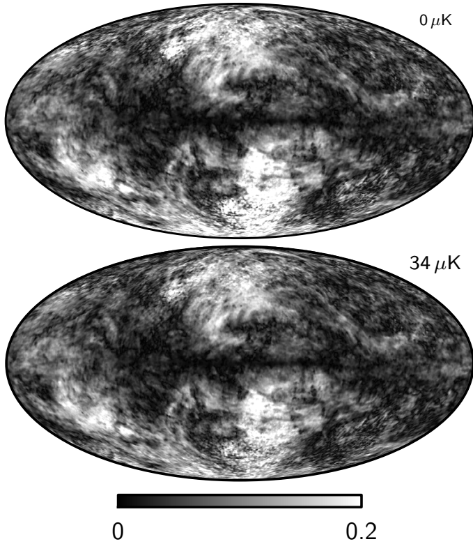
Fig. 43. Thermal dust polarization fraction for Galactic emission zero-level corrections of 0\mu\text{K} ( top ) and 34\mu\text{K} ( bottom ). A value of 34\mu\text{K} corresponds to our current best estimate of the residual zodiacal light offset in the 353 GHz channel (Planck Collaboration VIII 2016). The statistical uncertainty on the Galactic emission zero-level from HI cross-correlation is 0.0067\text{ MJy sr}^{-1} or 23\mu\text{K}_{\text{CMB}} .
