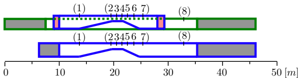
Fig. 7. Test setup for coupled case (upper schematic) and pure OpenFOAM case (lower schematic) for validation against experiments, OpenFOAM domain (blue outline) and OceanWave3D domain (green outline) in side view ( xz ). The numbers (1), (2)... mark the positions of numerical wave probes.
