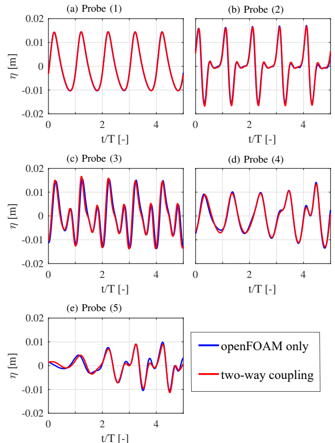
Fig. 10. Results of evaluation of a multi domain case, surface elevation over time normalised by wave period
