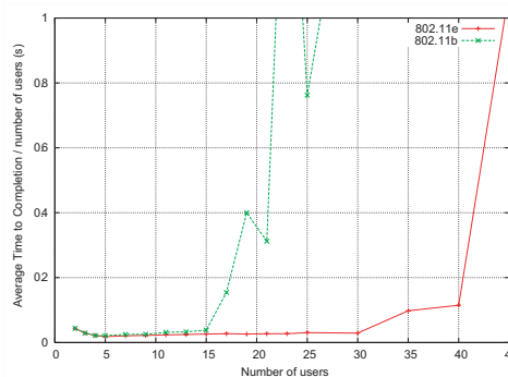
Fig. 3. Example of client-server performance in 802.11b and prioritised 802.11e WLANs.
