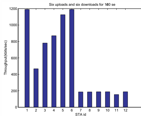
Fig. 1. Performance of six TCP uploads and six TCP downloads with default 802.11b parameters. Stations 1–6 are uploads and 7–12 are downloads.
