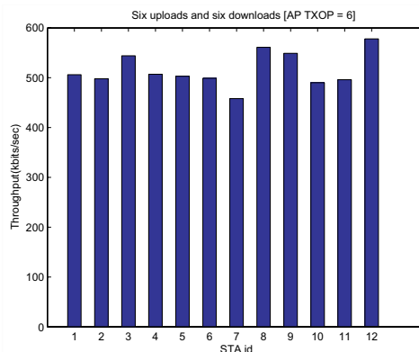
Fig. 2. Performance of six TCP uploads and six TCP downloads with suggested 802.11e parameters. Stations 1–6 are uploads and 7–12 are downloads.
