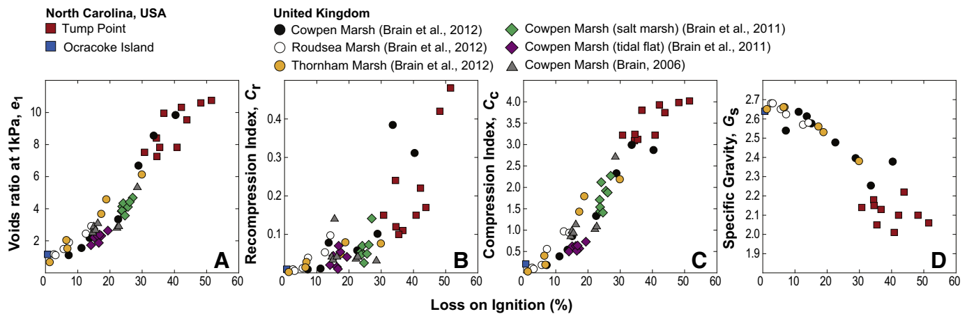
Figure 4. Observed relationships between geotechnical (A–C) and physical properties (D) of salt-marsh sediments used for model calibration. United Kingdom data are from Brain (2006), Brain et al. (2011) and Brain et al. (2012).
