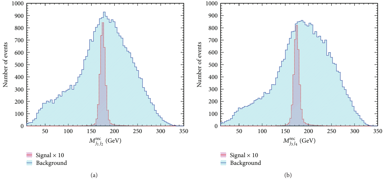
FIGURE 6: Reconstructed top quark mass distributions for the anomalous decay of both top quarks into a light quark and a gluon at \sqrt{s} = 0.5 TeV. The distributions are normalized to 100 \text{ fb}^{-1} integrated luminosity of data and for the signal \kappa_{tqg}/\Lambda = 0.02 \text{ TeV}^{-1} . The number of signal events is multiplied by a factor of 10.
