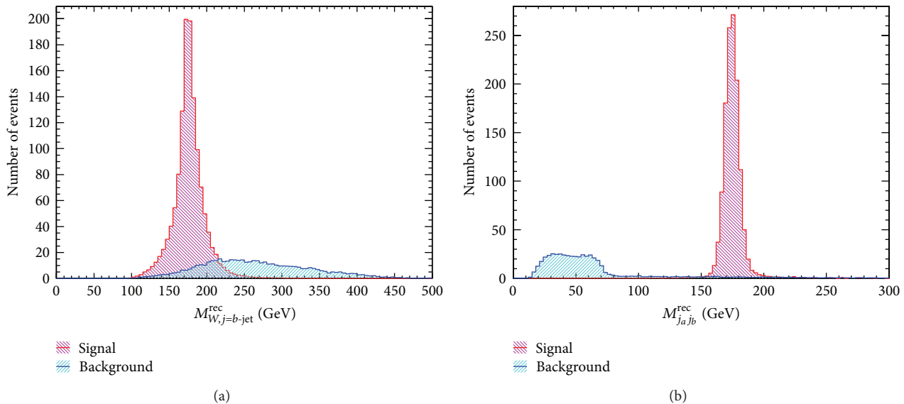
FIGURE 3: Reconstructed top quark mass distributions of the W boson and b -jet M_{W,jc=b\text{-jet}}^{\text{rec}} (a) and the other two-jet M_{ja,jb}^{\text{rec}} (b) after the preselection cuts, at \sqrt{s} = 0.5 TeV. The number of events is normalized to 100 \text{ fb}^{-1} integrated luminosity of data and for the signal \kappa_{tqg}/\Lambda = 0.02 \text{ TeV}^{-1} .
