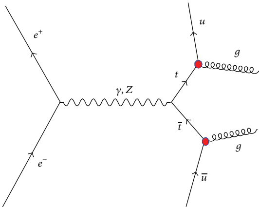
FIGURE 5: The representative Feynman diagram for the signal process in the hadronic channel.
