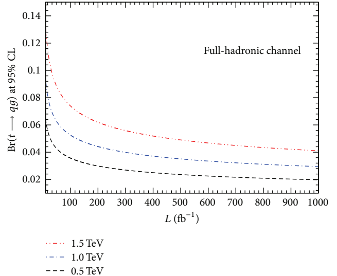
FIGURE 8: The 95% CL upper limits for \text{Br}(t \rightarrow qg) as a function of integrated luminosity for \sqrt{s} = 0.5, 1, and 1.5 TeV for the fully hadronic analysis.
