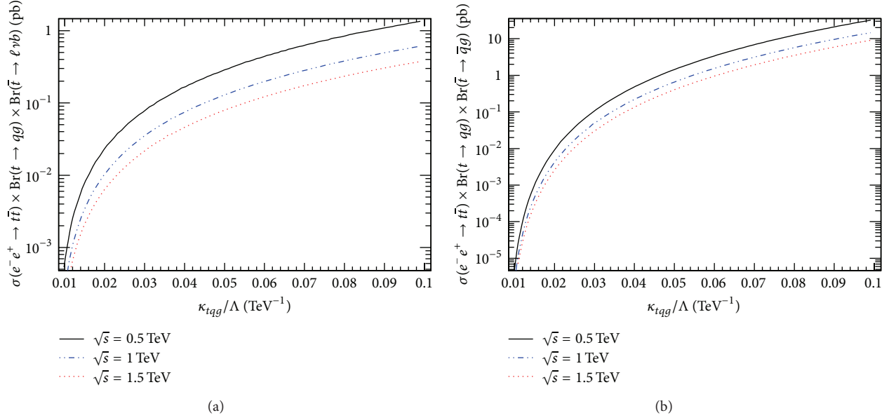
FIGURE 1: The cross section times branching ratio of one (a) and both (b) of the top quarks decay anomalously into q + g as a function of the anomalous coupling \kappa_{tqg}/\Lambda for \sqrt{s} = 0.5, 1, \text{ and } 1.5 TeV.
