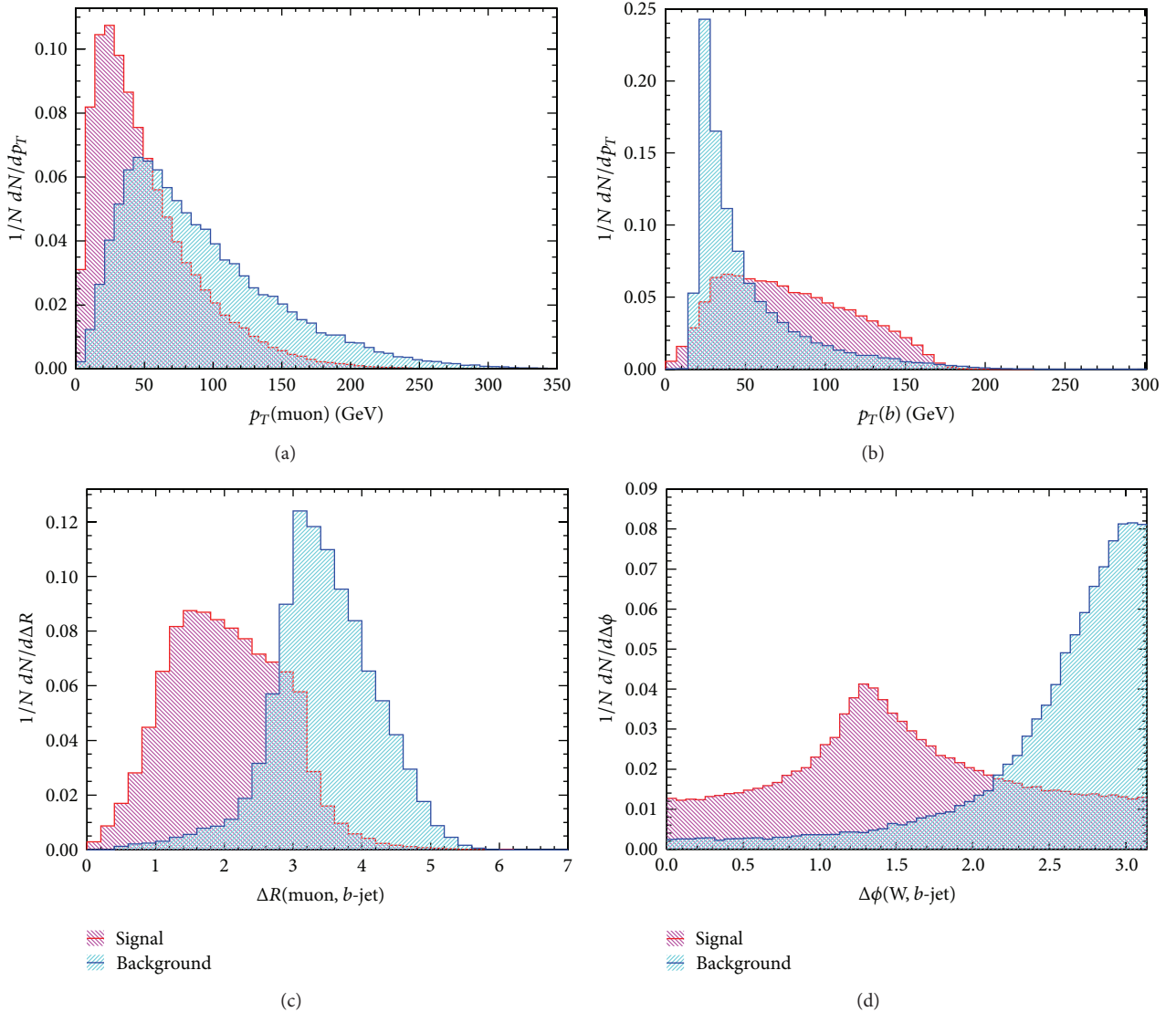
FIGURE 4: The kinematic distributions of four significance variables used as inputs to BDT in addition to the W boson and top mass distributions. (a) The transverse momentum of the charged lepton p_T(\ell) and (b) transverse momentum of the b -jet p_T(b) . (c) The angular separation between charged lepton and b -jet \Delta R_{\ell,b\text{-jet}} and (d) the difference of the azimuthal angle between the reconstructed W boson and the b -jet |\Delta\phi_{W,b\text{-jet}}| .
