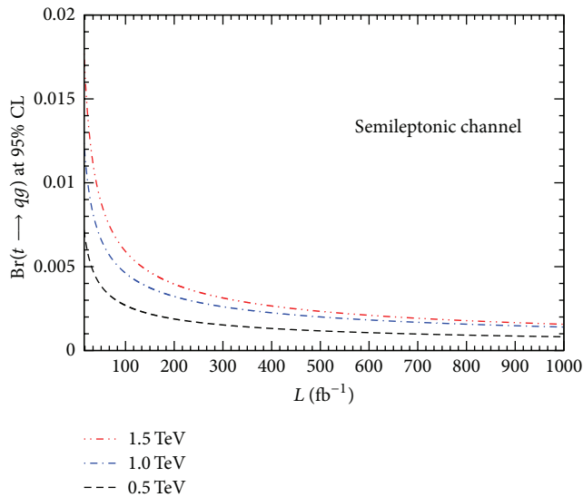
FIGURE 7: The 95% CL upper limits for \text{Br}(t \rightarrow qg) as a function of integrated luminosity for \sqrt{s} = 0.5, 1, and 1.5 TeV for the semileptonic analysis.
