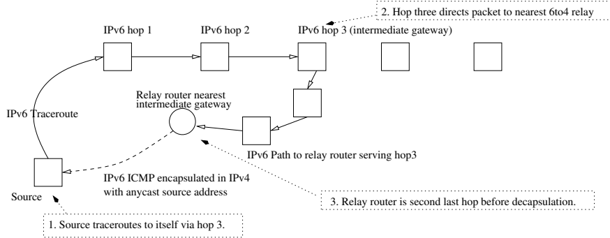
Figure 1: Identification of relay routers using IPv4 encapsulation address.
