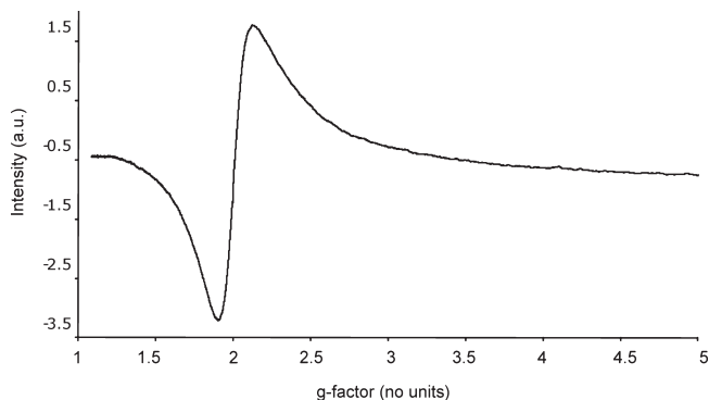
Figure 4. X-band (9.3896 GHz) CW EPR spectrum of a solid sample of 1 recorded at 296 K.
