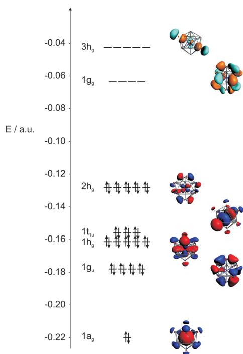
Figure 6. Kohn–Sham orbitals for icosahedral [\text{Ni}@\text{Pb}_{12}]^{2-} (contour value 0.025 au). Only one component of each degenerate orbital is shown.
