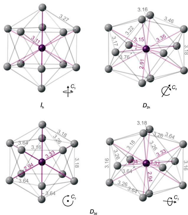
Figure 5. Optimized geometries of [\text{Mn}@\text{Pb}_{12}]^{3-} ( I_h , D_{2h} , and D_{3d} symmetries). Mn–Pb bonds and distances (Å) in purple, Pb–Pb bonds, and distances in gray. The orientation of the principal axis of rotation is indicated.
