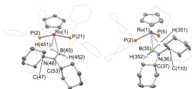
Figure 1. Structures of the cationic components of 5 and 6 . Anions and hydrogen atoms (except boron-bound hydrogens) are omitted, and phosphine substituents are shown in wireframe format for clarity. Thermal ellipsoids are set at the 30% probability level. Key bond lengths (Å) and angles (°): for 5 , Ru(1)–P(2) 2.354(1), Ru(1)–P(21) 2.358(1), Ru(1)···B(45) 2.430(4), Ru(1)–H(451) 1.665(4), B(45)–N(46) 1.376(4), B(45)–H(451) 1.207(4), B(45)–H(452) 1.114(4), Ru(1)···B(45)–N(46) 130.2(3); for 6 , Ru(1)–P(2) 2.338(1), Ru(1)–P(5) 2.319(1), Ru(1)···B(35) 2.332(6), Ru(1)–H(351) 1.669(1), B(35)–N(36) 1.382(7), B(35)–H(351) 1.244(6), B(35)–H(352) 1.150(5), Ru(1)···B(35)–N(36) 133.1(4). The boron-bound hydrogen atoms were located in the crystallographic Fourier difference maps.
