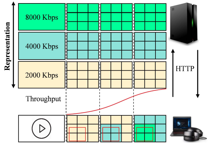
Fig. 8. Adaptive streaming of 3 \times 3 tiles of 360^\circ video with three segments and each containing one frame.
