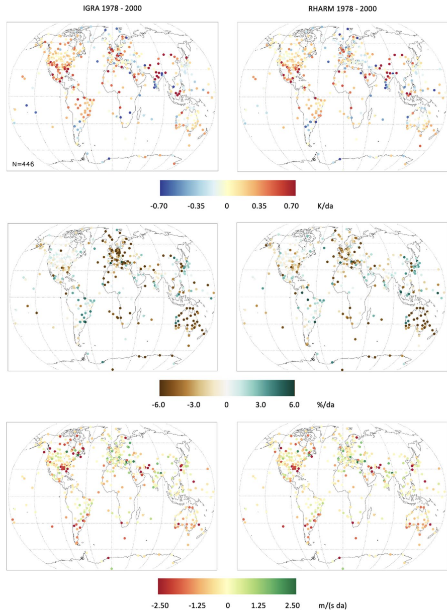
Figure 7. Global maps of the trends (per decade) at 300 hPa of temperature (top), relative humidity (middle) and wind speed (bottom) estimated from Integrated Global Radiosonde Archive (left panels) and Radiosounding HARMONization (right panels) stations. Trends have been estimated for each station in the period 1978–2000.
