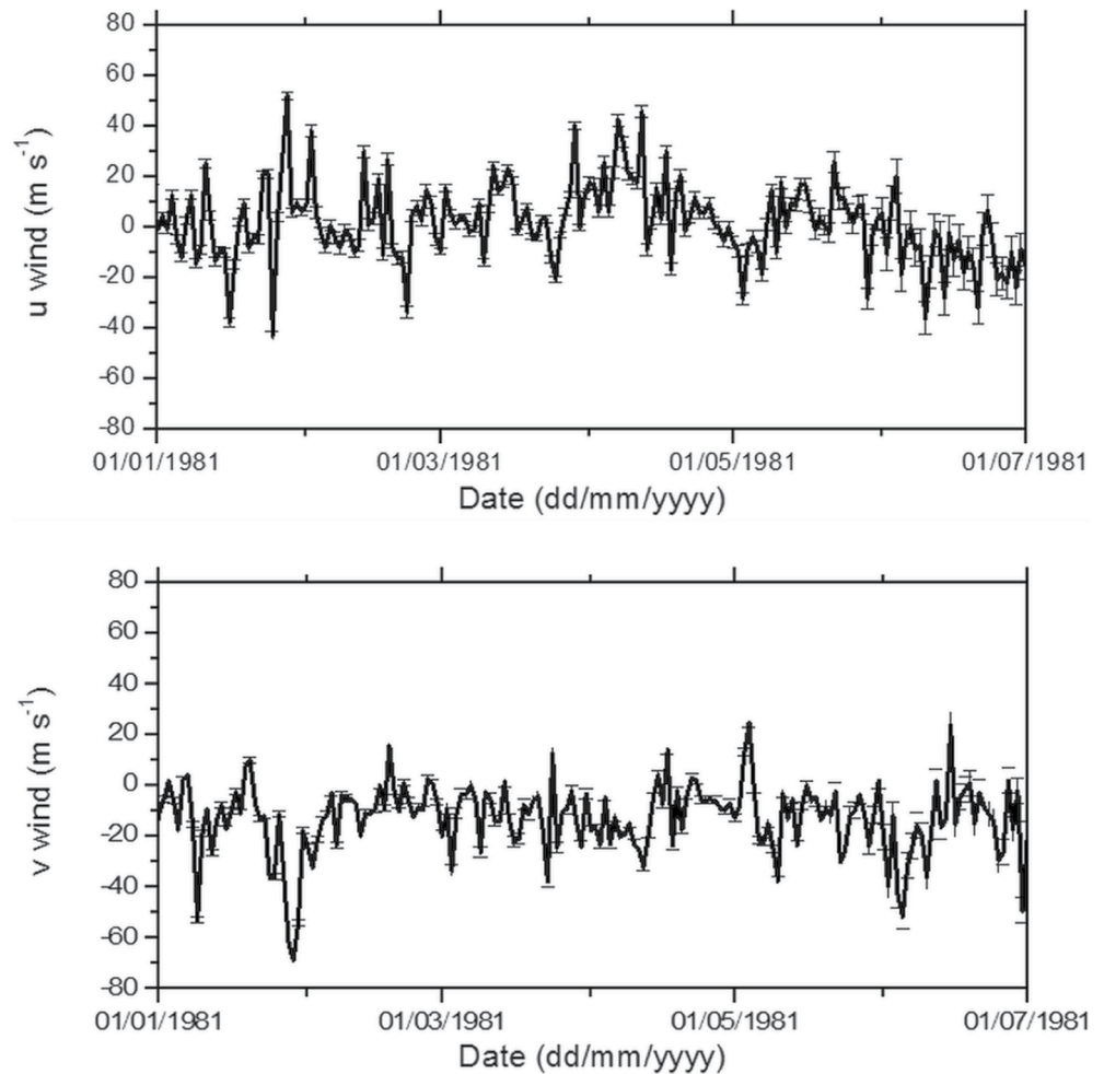
Figure A1. Top panel, zonal wind component ( u ) time series at 300 hPa (only nighttime) for the Sodankyla station with the uncertainties calculated using Radiosounding HARMonization for the period from 01/01/1981 to 01/07/1981. Bottom panel, same as top panel but for meridional component ( v ). The vertical bars show the random uncertainties quantified using the statistical method, and their plotting has been reduced to one value each two of the time series.
