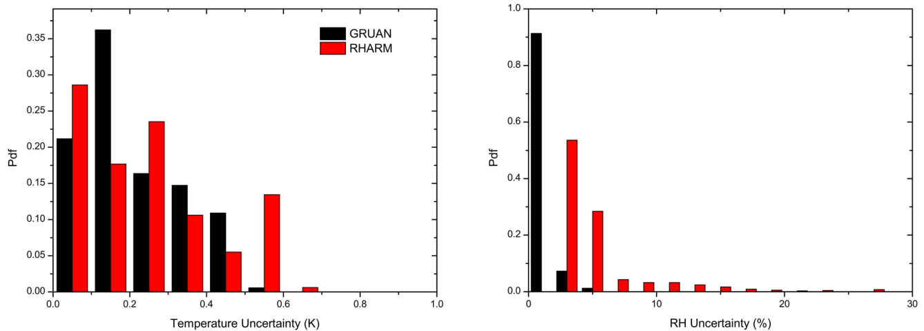
Figure 15. Comparison of pdfs of the uncertainty calculated using the Global Climate Observing System (GCOS) Reference Upper Air Network data processing and the Radiosounding HARMONization approach at the six stations shown in Table 1. Pdfs are relative to temperature (panel a) and relative humidity (panel b).
