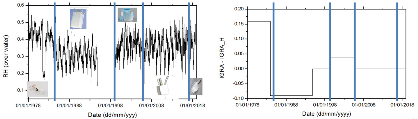
Figure 5. Left panel, relative humidity monthly time series for the station of Sodankyla (World Meteorological Organization [WMO] index = 2,836, 67.3667 N 26.6289 E, 179 m asl) as available from Integrated Global Radiosonde Archive (IGRA), reporting the radiosonde pictures used in different periods delimited by blue lines. Right panel, adjustments applied by the Radiosounding HARMonization (RHARM) algorithm (IGRA minus RHARM) with blue lines indicating sensor changes as in the left panel.
