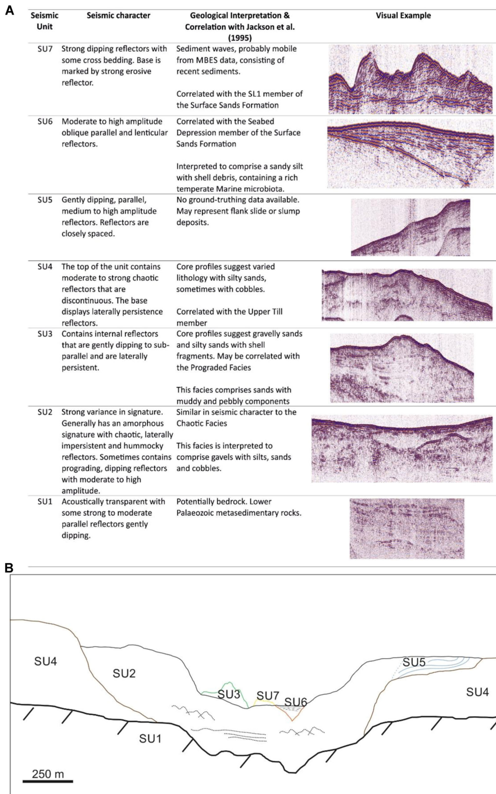
Figure 4. A: Description of seismic units found in Wicklow Trough sparker seismic profiles with correlation to the previous stratigraphic framework of Jackson et al. (1995). B: Composite representative stratigraphic cross-section of the Wicklow Trough. [Color figure can be viewed at wileyonlinelibrary.com ]
