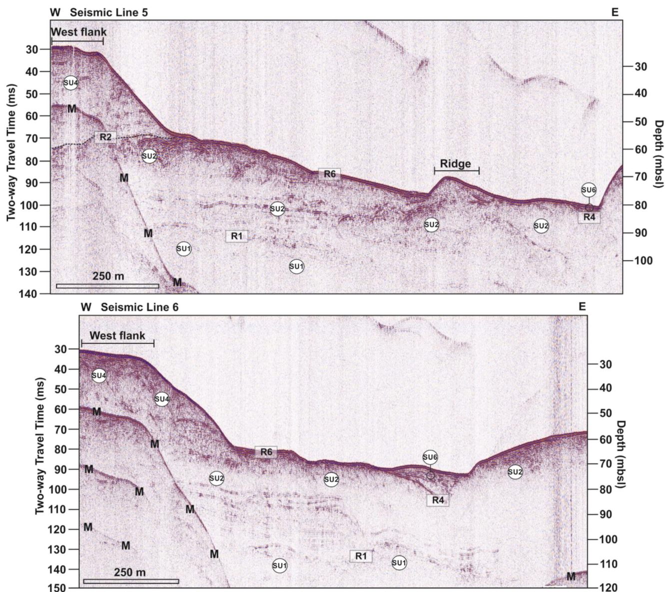
Figure 7. Seismic line 5 (SL5) and SL6 with seismo-stratigraphic interpretation. Depth is presented in two-way travel time and metres below sea-level (mbsl). 'M' indicates seabed multiple. [Color figure can be viewed at wileyonlinelibrary.com ]
