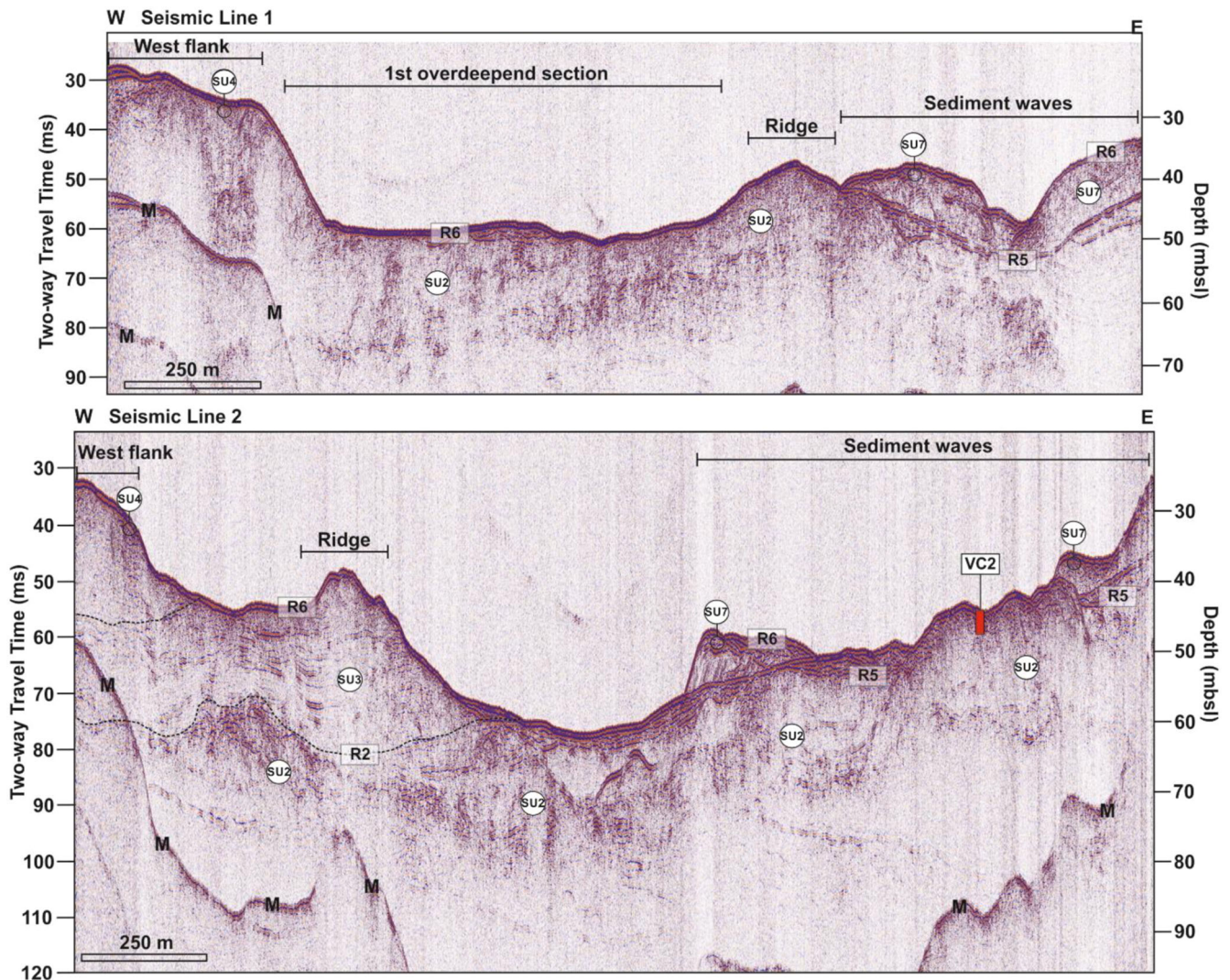
Figure 5. Seismic line 1 (SL1) and SL2 with seismo-stratigraphic interpretation and core locations with depth. Depth is presented in two-way travel time and metres below sea-level (mbsl). 'M' indicates seabed multiple. [Color figure can be viewed at wileyonlinelibrary.com ]
