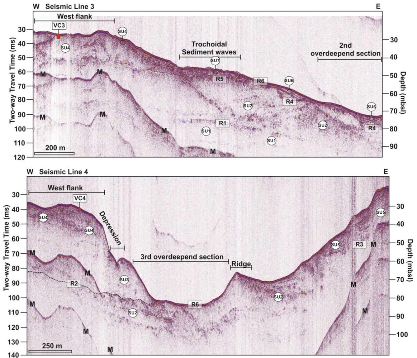
Figure 6. Seismic line 3 (SL3) and SL4 with seismo-stratigraphic interpretation and core locations with depth. Depth is presented in two-way travel time and metres below sea-level (mbsl). 'M' indicates seabed multiple. [Color figure can be viewed at wileyonlinelibrary.com ]
