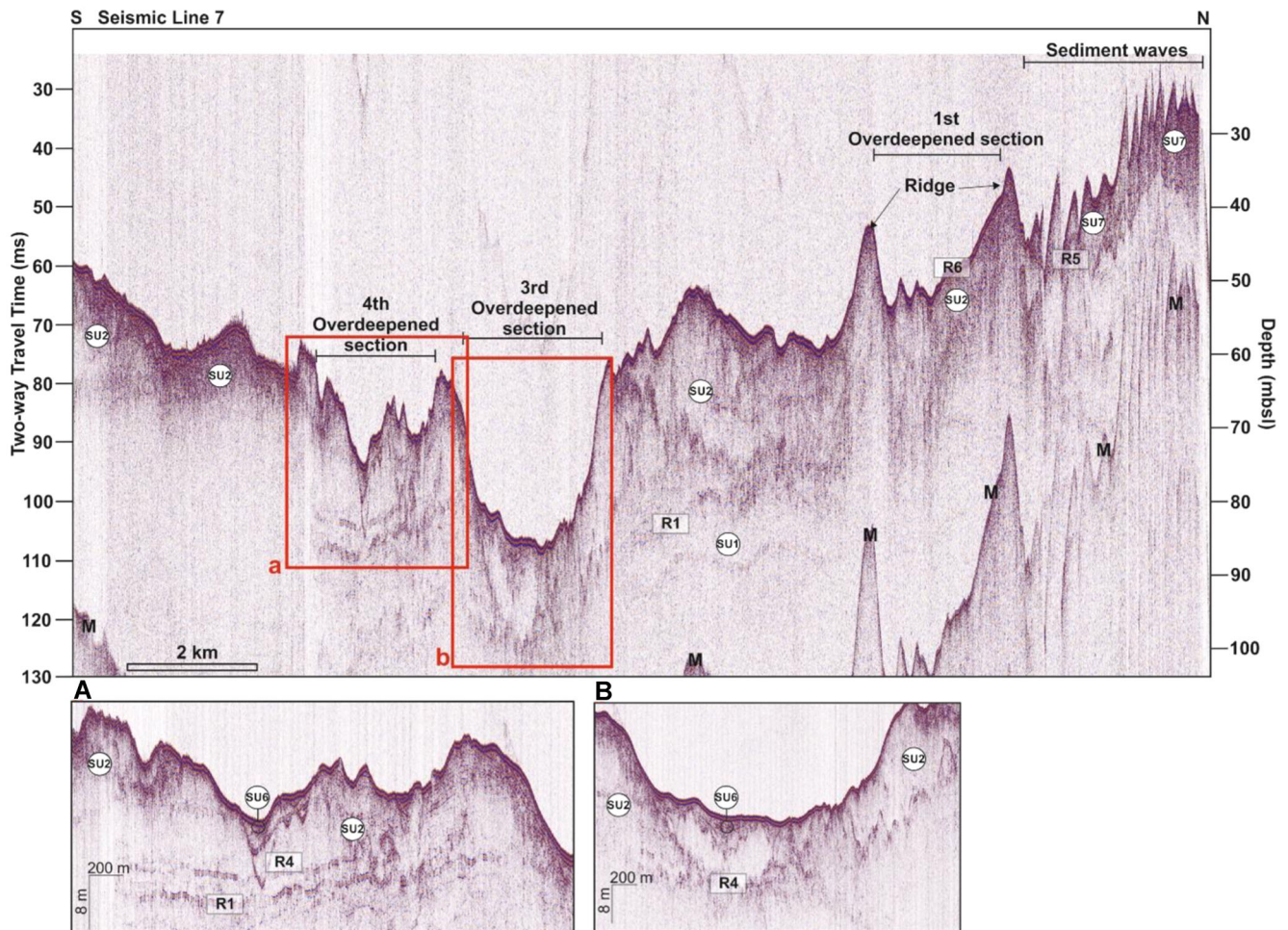
Figure 8. Seismic line 7 (SL7) with seismo-stratigraphic interpretation with highlighted features. Depth is presented in two-way travel time and metres below sea-level (mbsl). 'M' indicates seabed multiple. [Color figure can be viewed at wileyonlinelibrary.com ]
