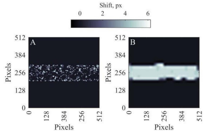
Figure 34. PIV (particle image velocimetry) analysis of simulated subjective speckle pattern. (A) Uneven ‘boiling’ of a speckle field in focal plane. (B) Uniform shift in one direction with predicted magnitude of 6 pixels. Three passes PIV algorithm with decreasing interrogation/searching windows 128/256, 64/128, 32/64 and threshold value of 0.6 were used to compute both images.
