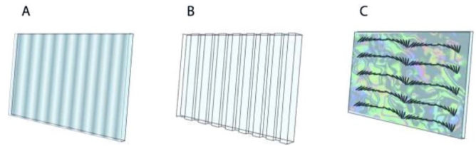
Figure 26. Schemes of different types of diffraction gratings produced by means of holography: (A) VPHG (periodic modulation of the refractive index); (B) HSRG (periodic modulation of the thickness); (C) PG (based on liquid crystals technology).
