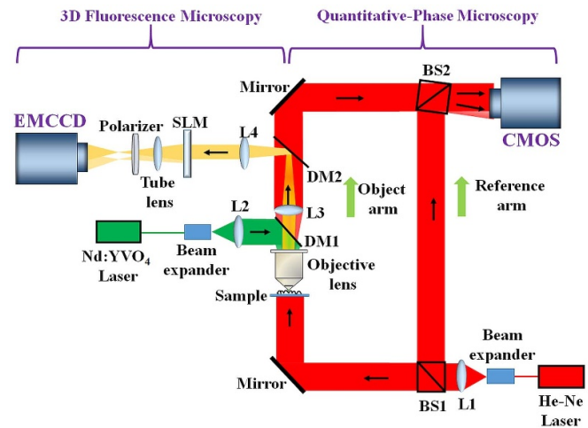
Figure 13. The schematic of the multimodal imaging system.
