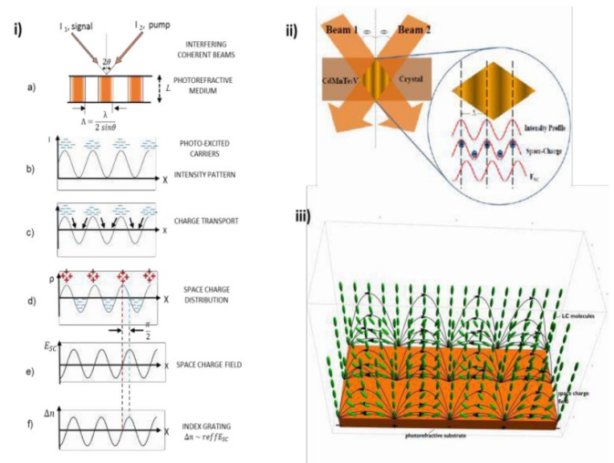
Figure 8. Schematic diagram of (i) photorefractive effect, (ii) two-beam coupling in an inorganic crystal. Reprinted with permission from [54] © The Optical Society. (iii) Penetration of space-charge field in organic-inorganic hybrid structure. [55] John Wiley & Sons. © 2016 WILEY-VCH Verlag GmbH & Co. KGaA, Weinheim.
