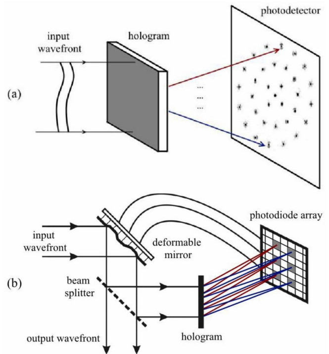
Figure 17. Modal holographic WFS (a) and AO system with zonal holographic WFS (b).
