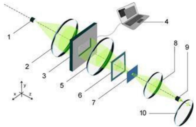
Figure 11. Projection scheme for recording computer-synthesized 2D Fourier holograms. 1—radiation source (LED), 2—collimating lens; 3—SLM; 4—personal computer; 5—Fourier lens; 6—analyzer; 7—aperture; 8—lens; 9—micro lens; 10—holographic media (disk).
