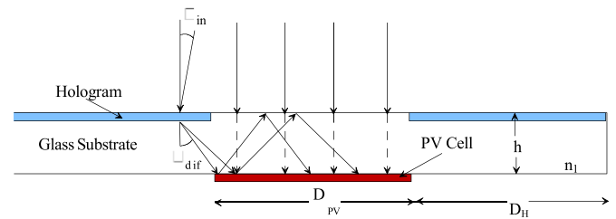
Figure 10. Holographic planar concentrator showing light collected by the hologram directed to the PV cell. Reproduced with permission from [128].
