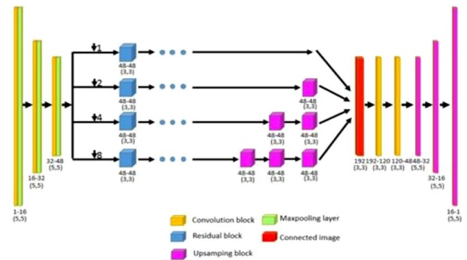
Figure 32. Typical neural network architecture for holographic reconstruction. Reprinted with permission from [308] © The Optical Society.
