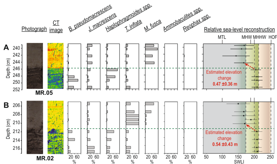
Figure 10. Plots showing Mad River Slough stratigraphy of the ca. 1120 cal a BP earthquake at three core sites: A. MR.14.05; B. MR.14.02. The plots include photo images, CT scans (rainbow scale; warm colours = more dense and cool colours = less dense), percentage foraminifera (grey bar) and results of BTF-reconstructed sea level with error bars that represent 1\sigma uncertainties. HOF: highest occurrence of foraminifera. SWLI: standardised water-level index. [Color figure can be viewed at wileyonlinelibrary.com]
