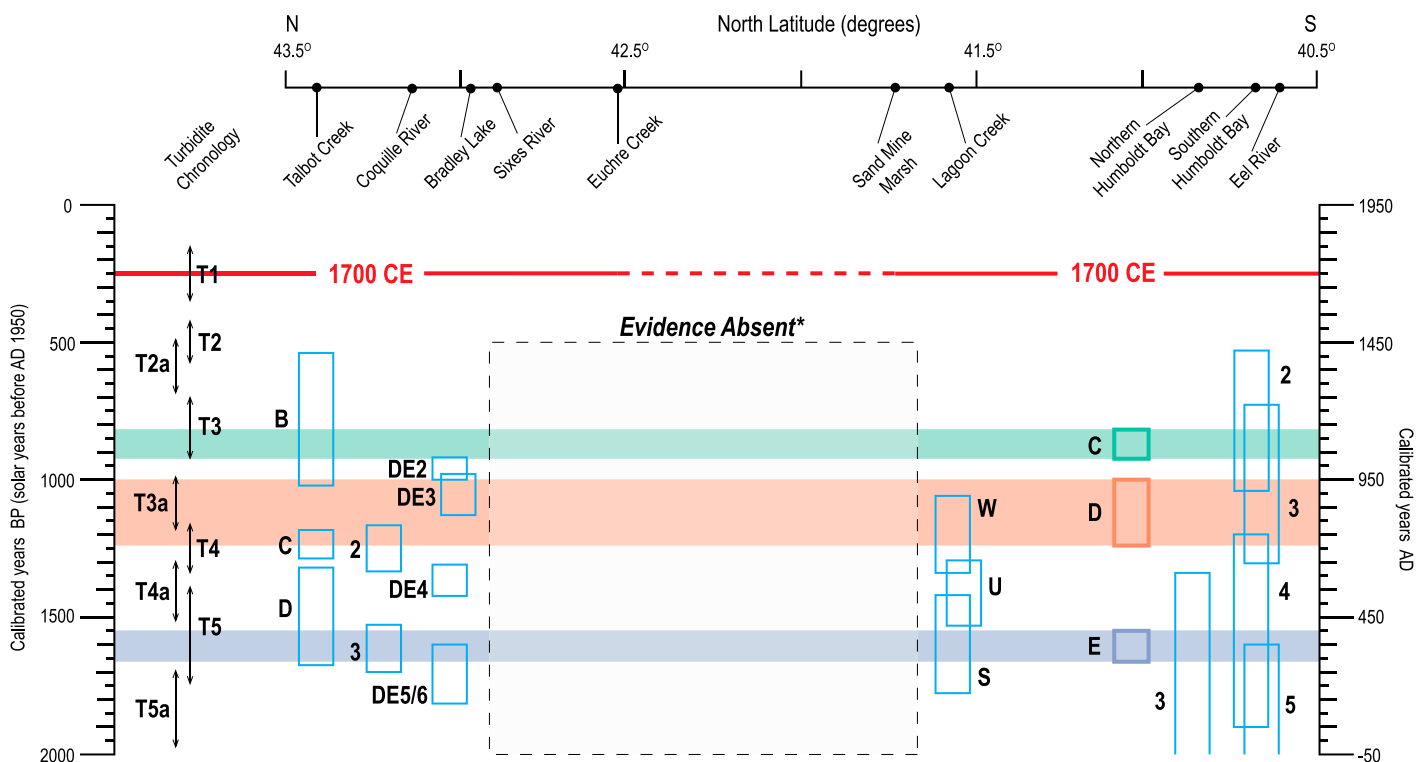
Figure 6. Comparison of dated mud-over-peat and mud-over-upland soil contacts beneath southern Cascadia salt marshes (Talbot Creek: Milker et al., 2016; Coquille River: Witter et al., 2003; Southern Humboldt Bay: Patton, 2004; Eel River: Li, 1992) and tsunami deposits at Lagoon Creek (Abramson, 1998; Garrison-Laney, 1998) and Bradley Lake (Kelsey et al., 2005) are shown with OxCal Sequence-modeled timing of subsidence contacts for northern Humboldt Bay and ages of marine turbidites (vertical black arrows show 2σ uncertainties from Goldfinger et al., 2012). Evidence Absent* —To date, evidence of coseismic subsidence in the time range ca. 500–2000 yr B.P. has not been found in the latitude range 41.7°–42.9°N. Absence of evidence may be because megathrust slip was insufficient to cause vertical deformation to be recorded by the salt marsh and/or because vertical deformation was further offshore and only minimal vertical deformation occurred at coastal sites. Further field work in salt marshes may reveal subsidence stratigraphy for the time and latitude range above.
