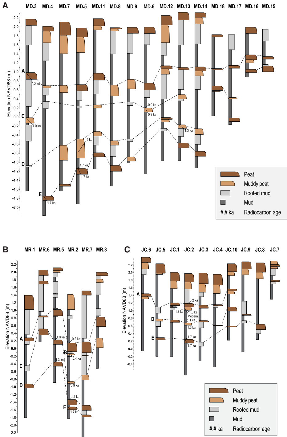
Figure 3. Simplified lithostratigraphy of northern Humboldt Bay at (A) McDaniel Creek, (B) Mad River Slough, and (C) Jacoby Creek. Core depths are shown relative to present-day elevation. Calibrated 14 C ages (ka; mode of 14 C distribution rounded to the nearest century) are shown for samples above and below contacts (more complete radiocarbon age data in Table 2). The letters A, B, C, D, and E refer to submergence contacts that are tested to be evidence for megathrust-induced subsidence. See Table 2 for more complete radiocarbon age data.
