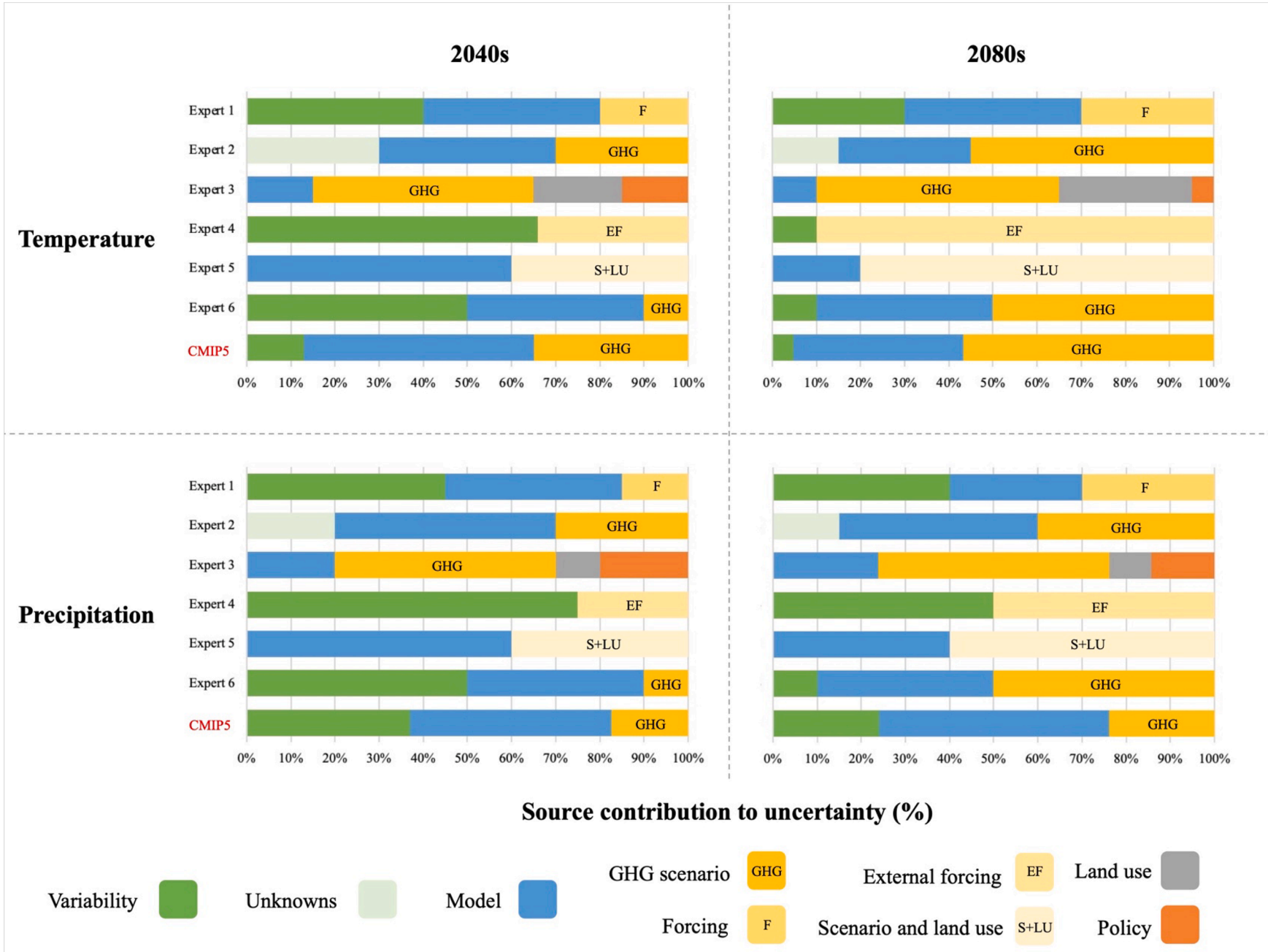
Fig. 3. Expert judgements of the percentage contribution to overall uncertainty when estimating mean annual temperature (top) and precipitation (bottom) for the 2040 s (left) and 2080 s (right) in the Lower Yangtze region, China. Bottom bars represent source contribution to uncertainty calculated using mean annual CMIP5 results for the Lower Yangtze domain.
