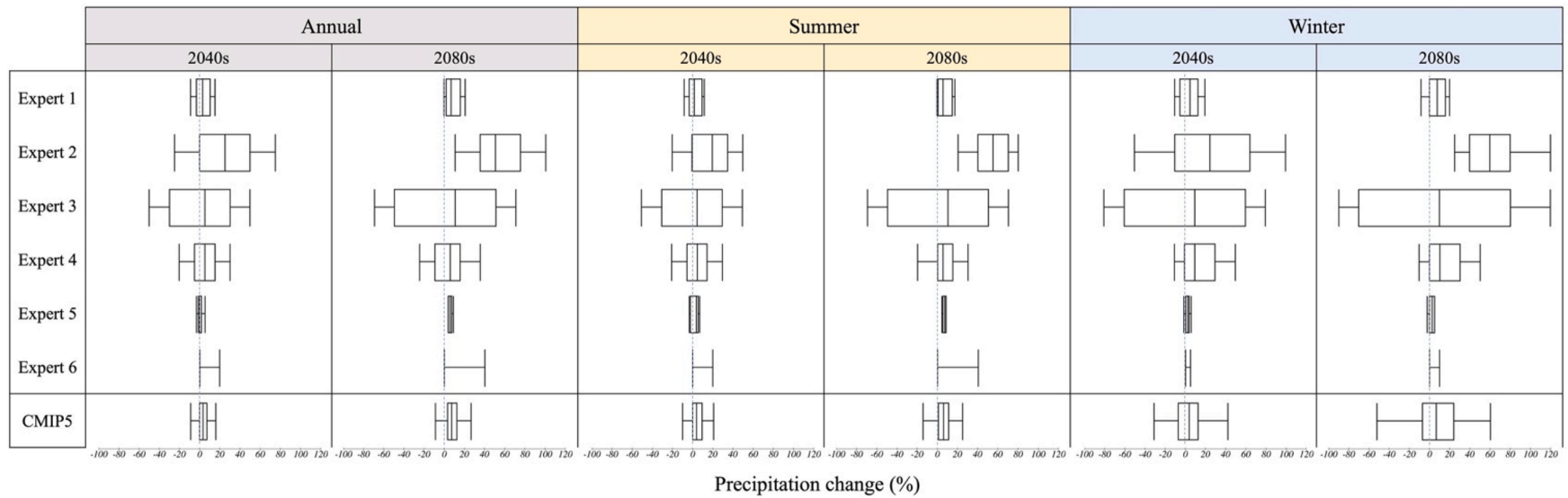
Fig. 2. Boxplots of future climate change in the Lower Yangtze region, China. For each plot, the first line to the left denotes the minimum value; the left vertical line of the box denotes first quartile; the internal vertical line denotes the median value, the right vertical line of the box denotes the third quartile; and the far right of the box denotes the maximum value.
