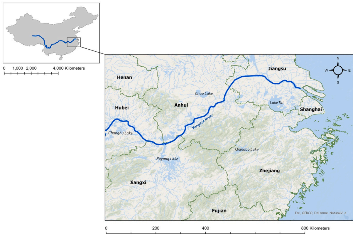
Fig. 1. The Lower Yangtze region of China (27°N to 33°N, 114°E to 123°E). The bold blue lines represent the main channel of the Yangtze River. Green shading represents higher elevation areas.
