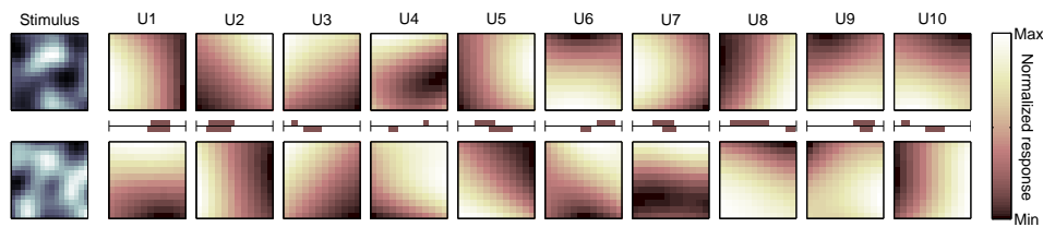
Figure 5.2: Activity of model units was modulated by the attentional signal. Color-coded images represent the activity of each bottleneck unit for a fixed stimulus as the center of attention is directed to different regions of the input space. Two different stimuli (top and bottom rows) are used for comparison. Maps are scaled according to the range of activities observed for that particular stimulus. The bars between the two rows display the range of activity for each of the two conditions with respect to the absolute limits of the activity of the units.
